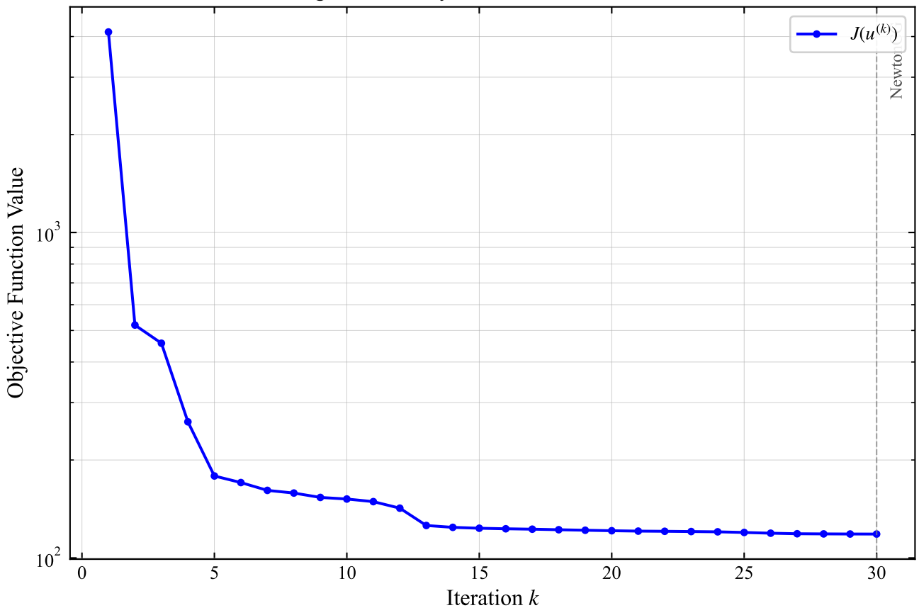
Convergence History — NewtonCG+GradDescent
