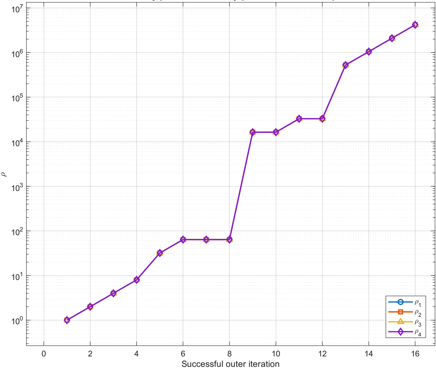
Penalty parameters history (successful iterations)
