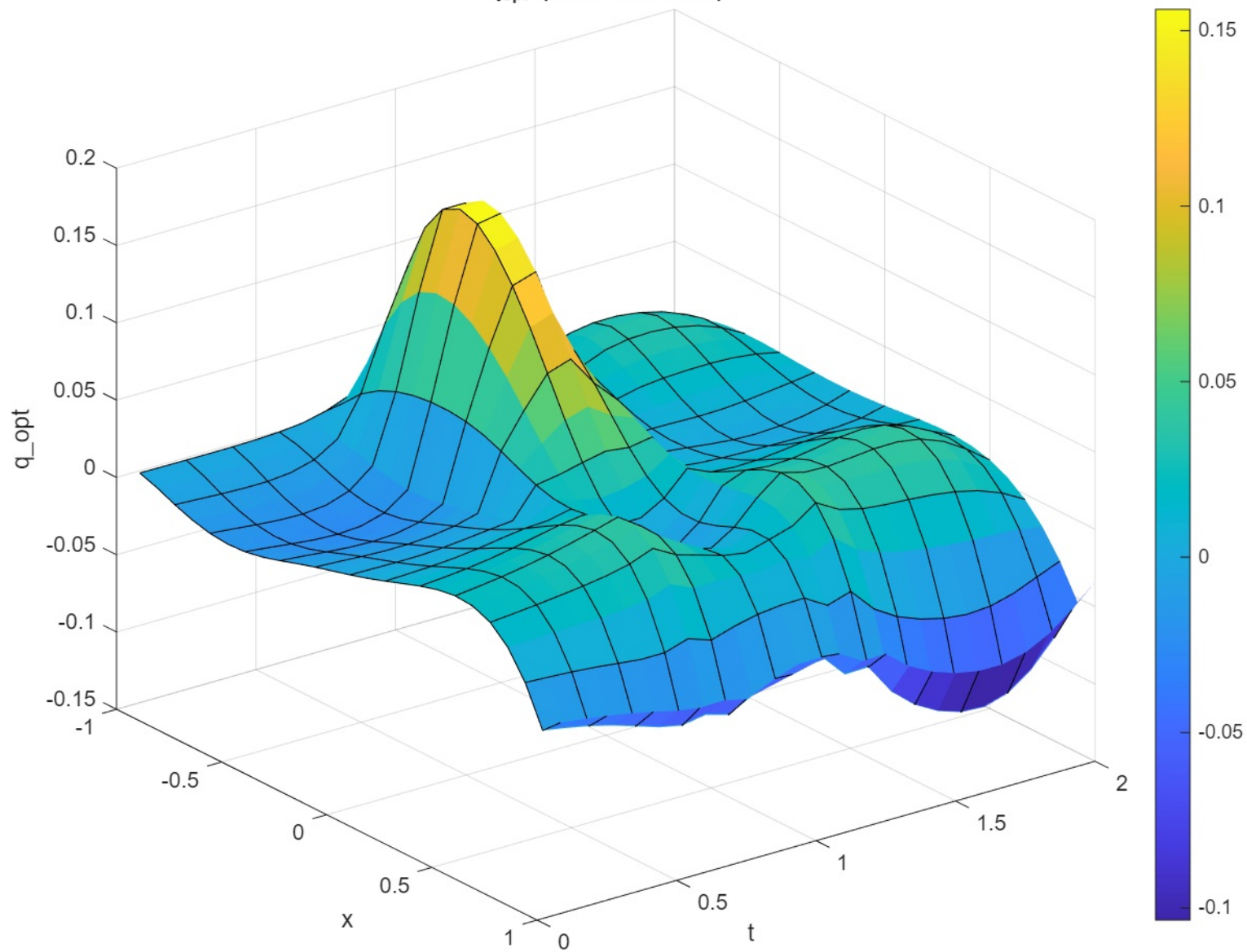
q_{\text{opt}} (Unconstrained)
