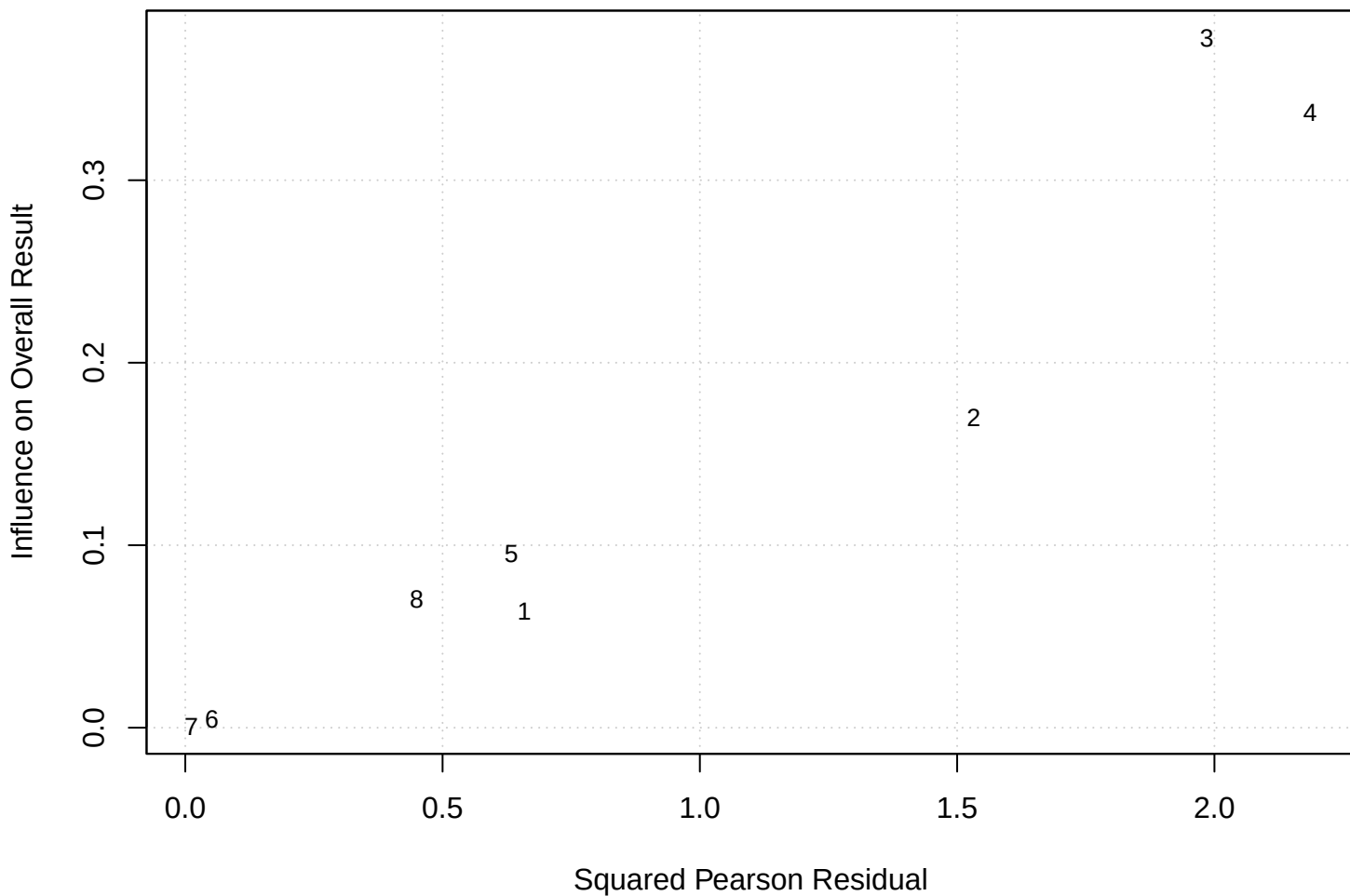
Baujat Plot: Contribution to Heterogeneity
