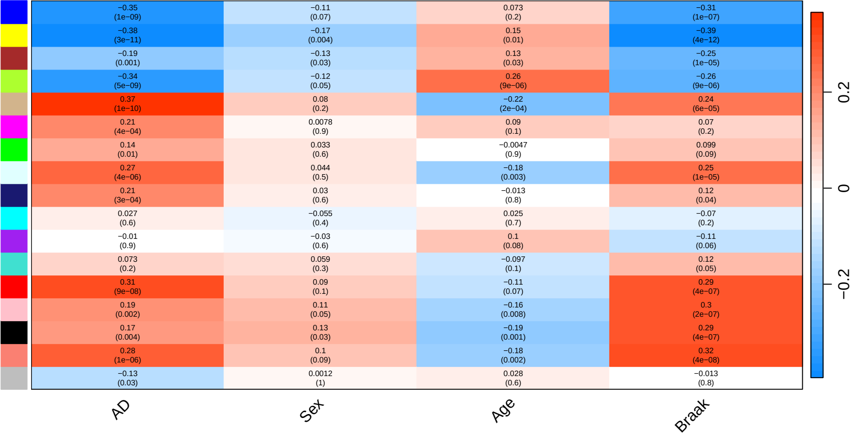
Module-trait relationships in GSE125583
