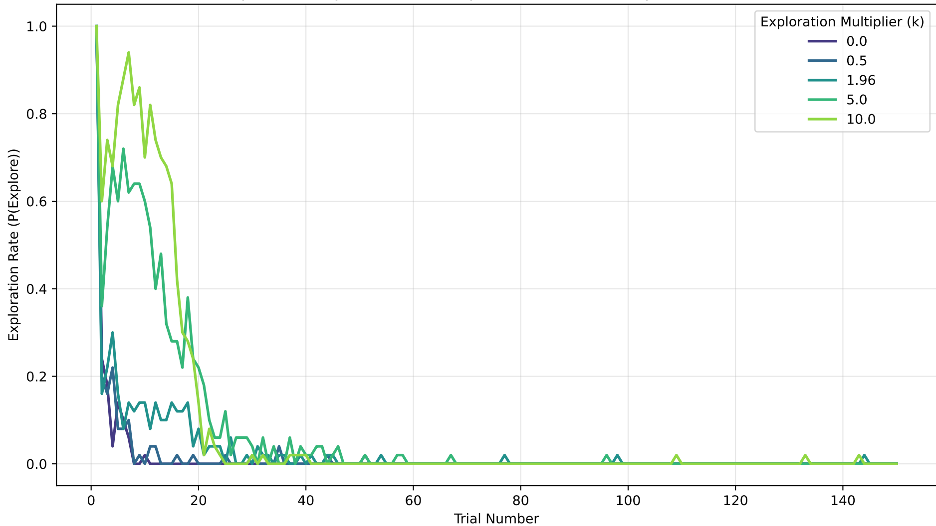
Impact of Exploration Multiplier (k) on UCB Exploration Rate
