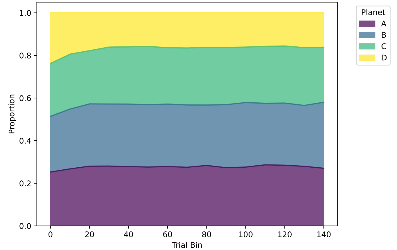
Planet Selection Frequency over Trials (Binned)
