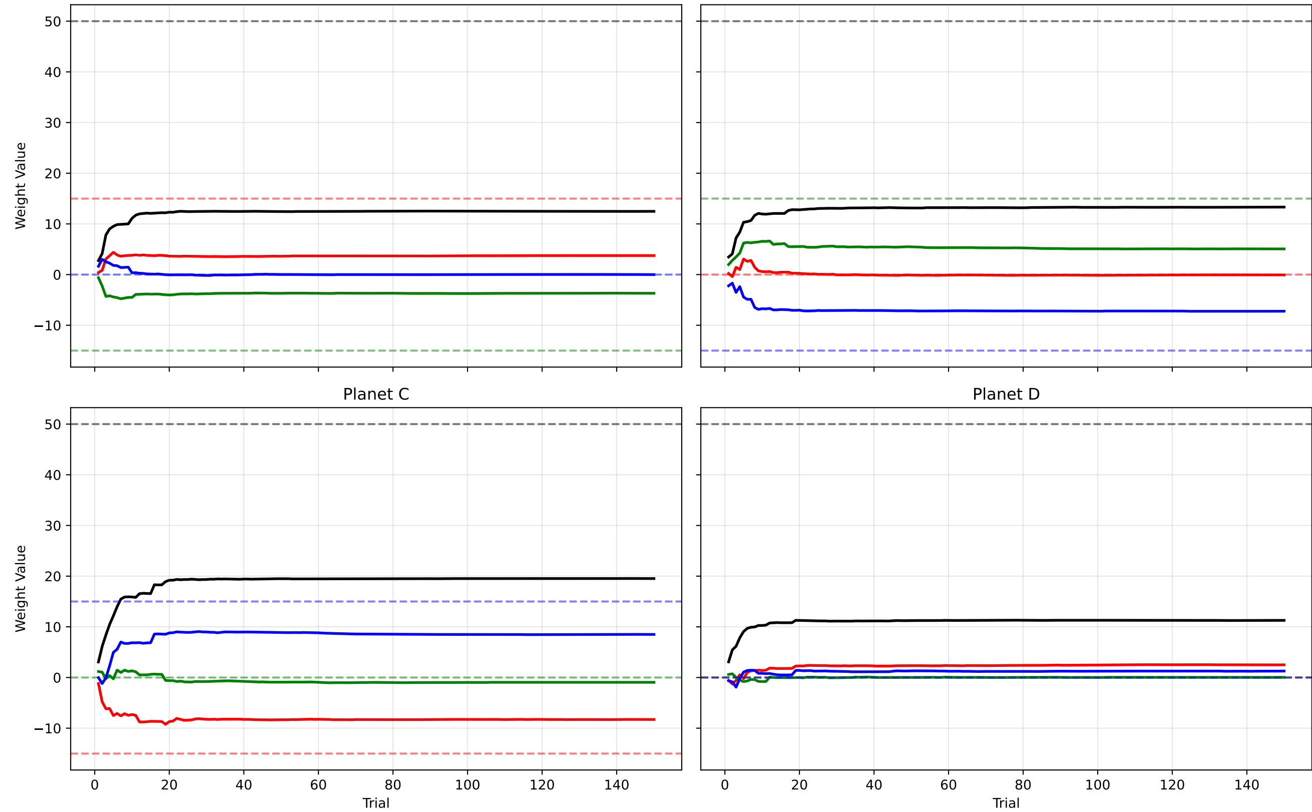
Planet A
