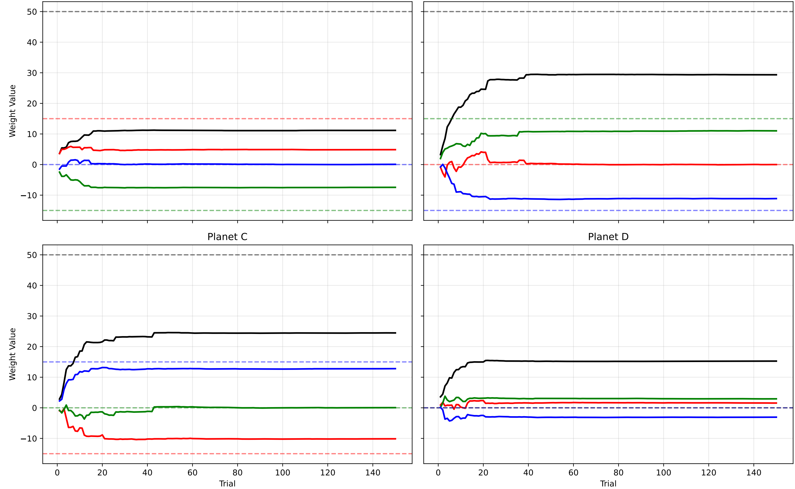
Planet A
