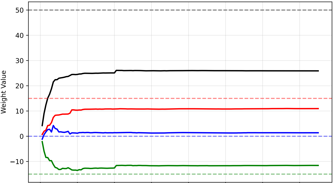
Planet A
