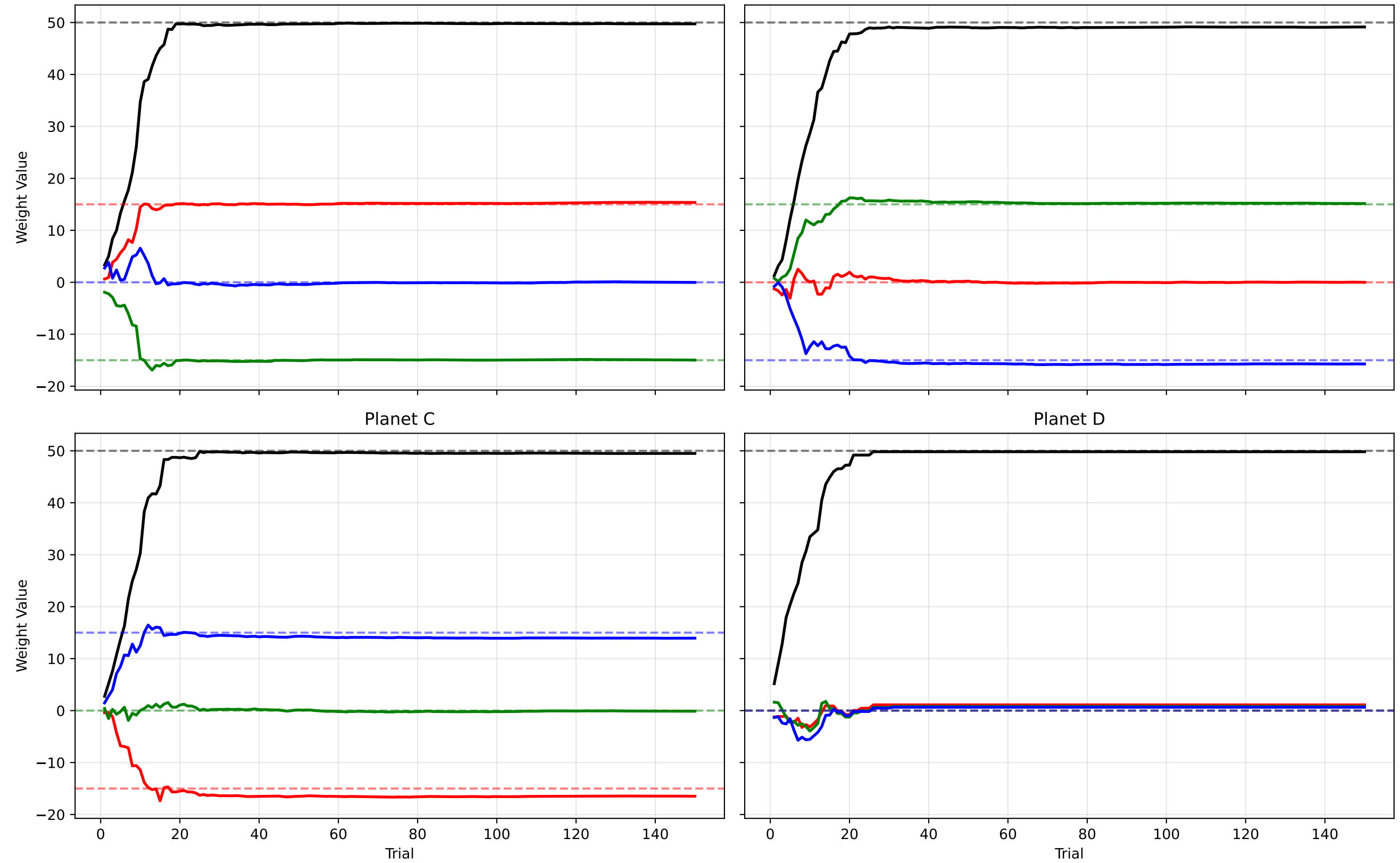
Planet A
