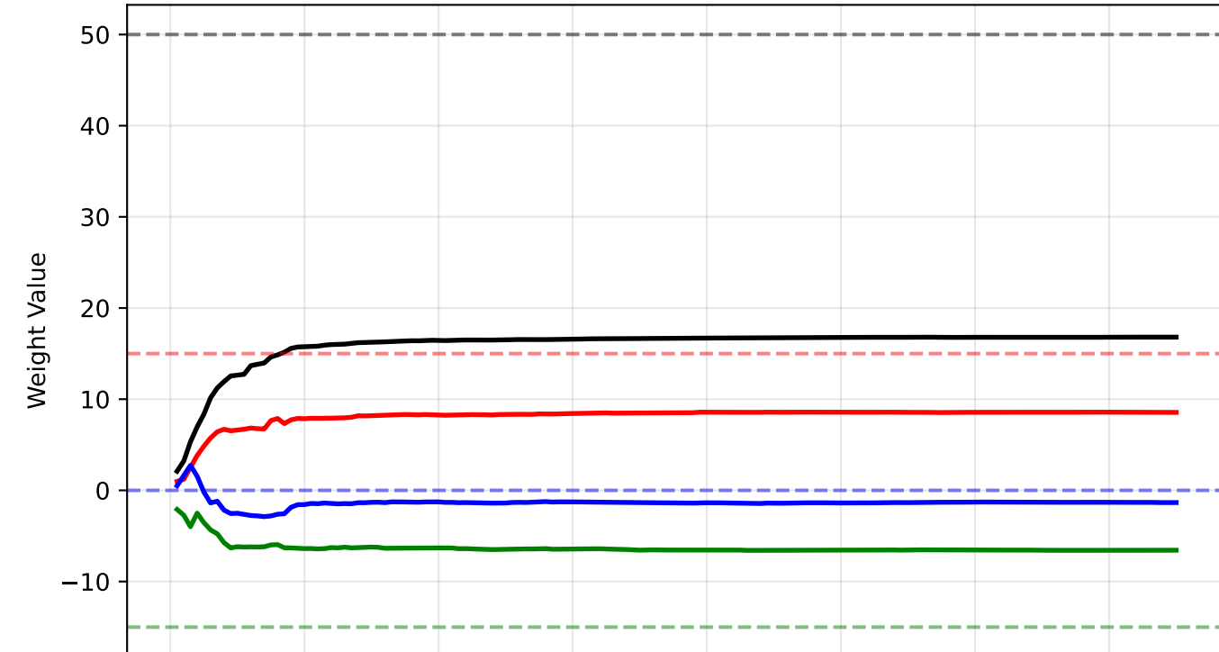
Planet A
