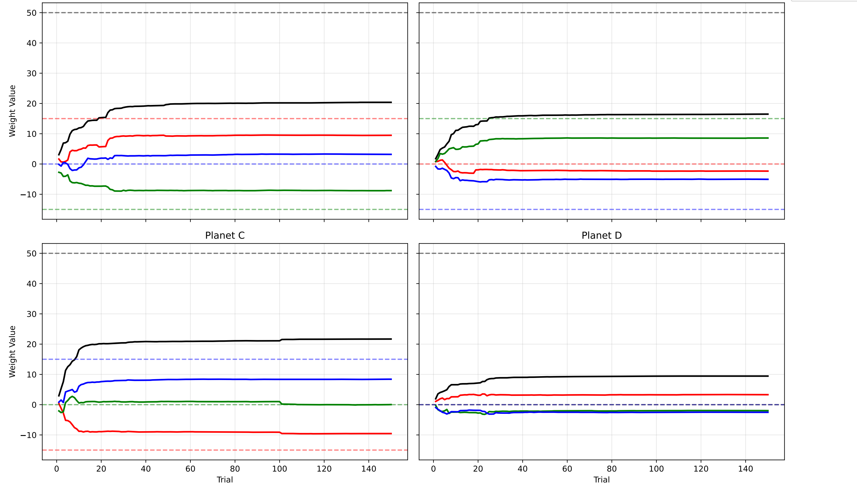
Planet A
