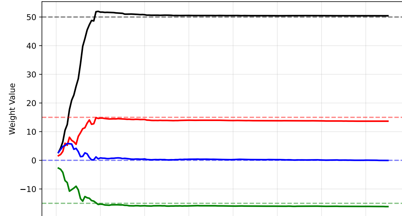
Planet A
