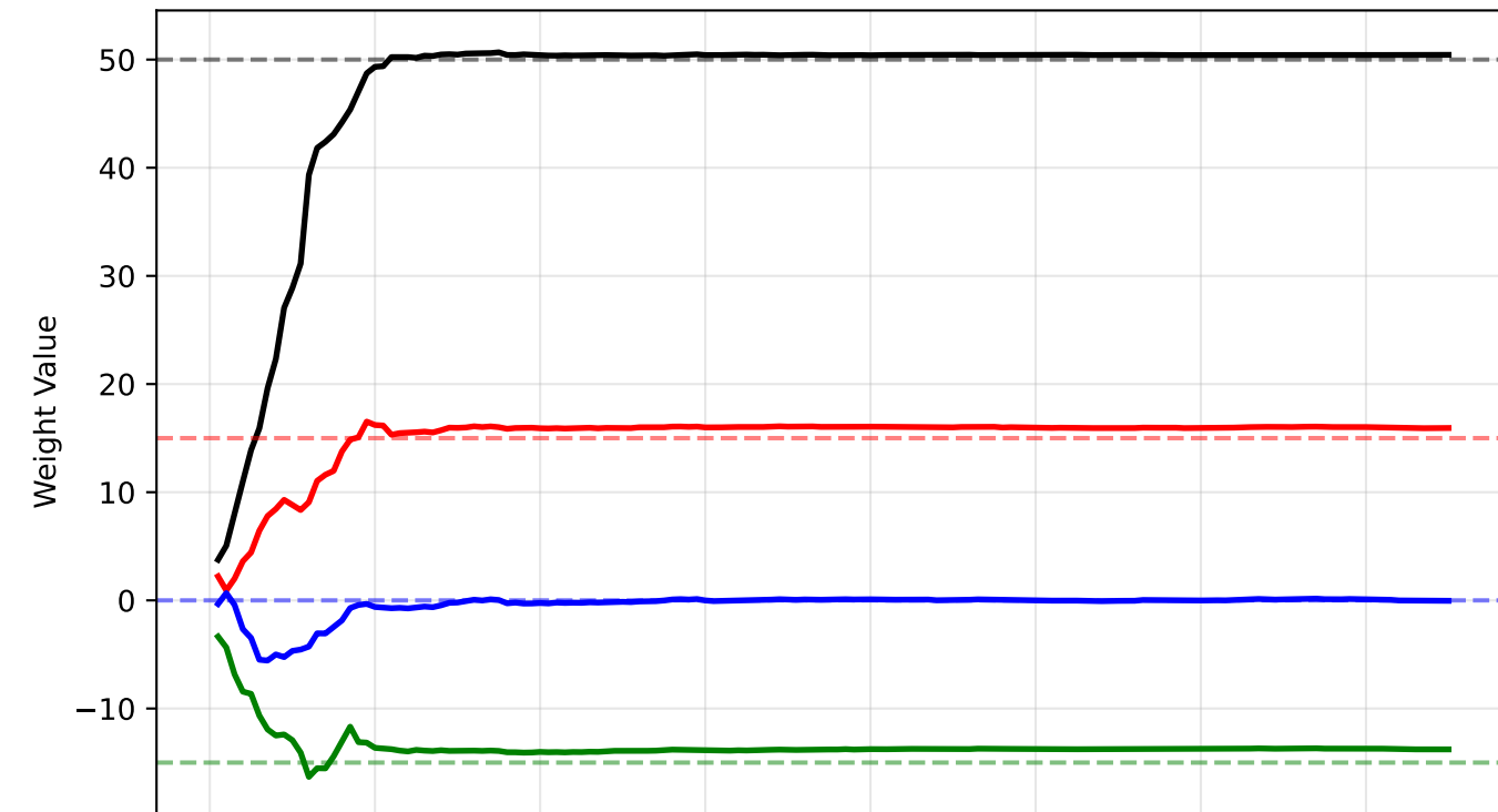
Planet A
