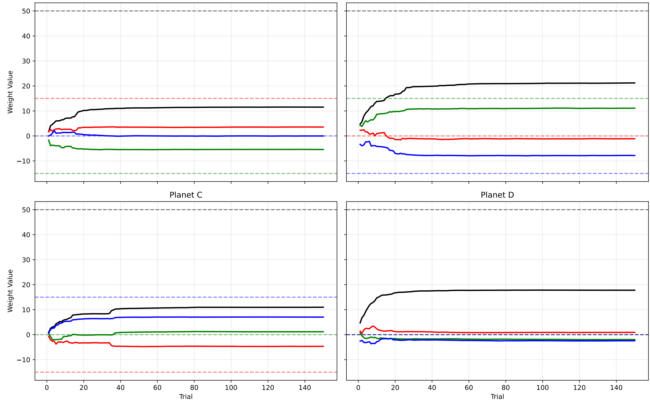
Planet A
