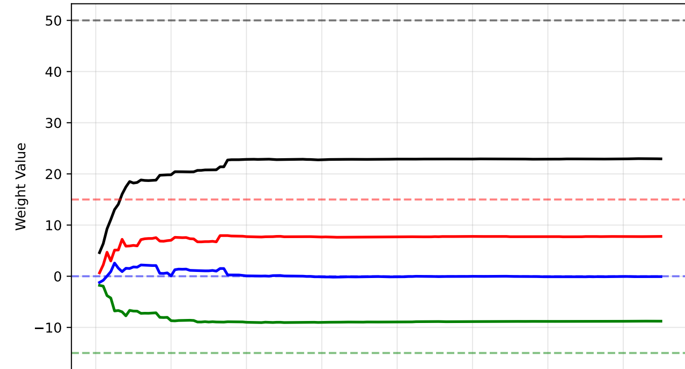
Planet A
