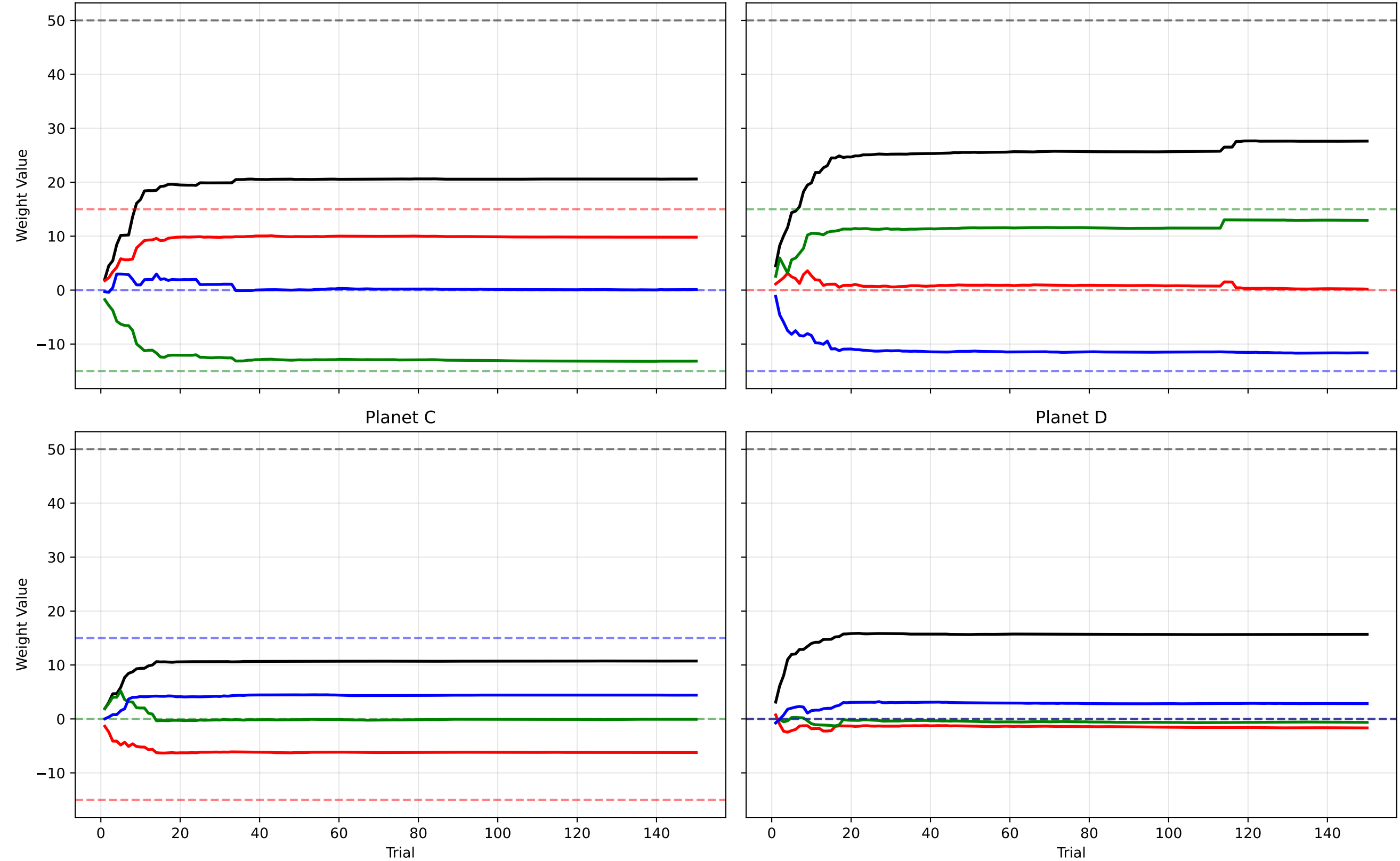
Planet A
