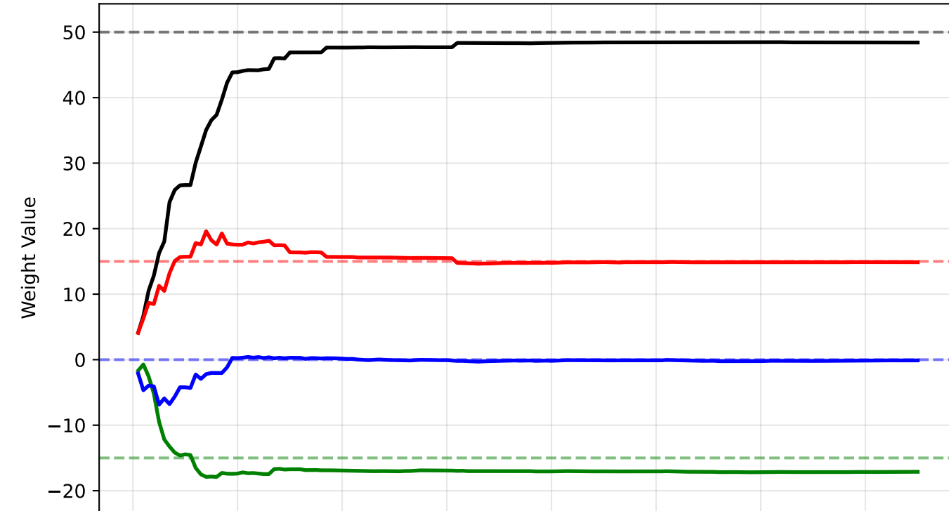
Planet A
