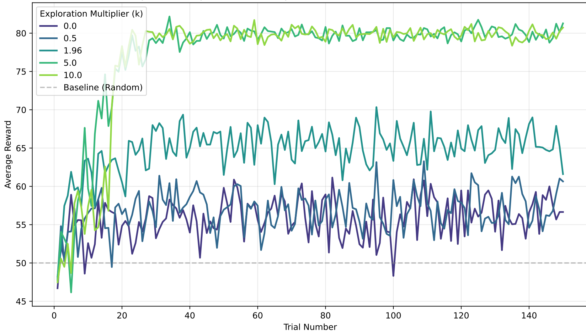
Impact of Exploration Multiplier (k) on Linear UCB Performance
