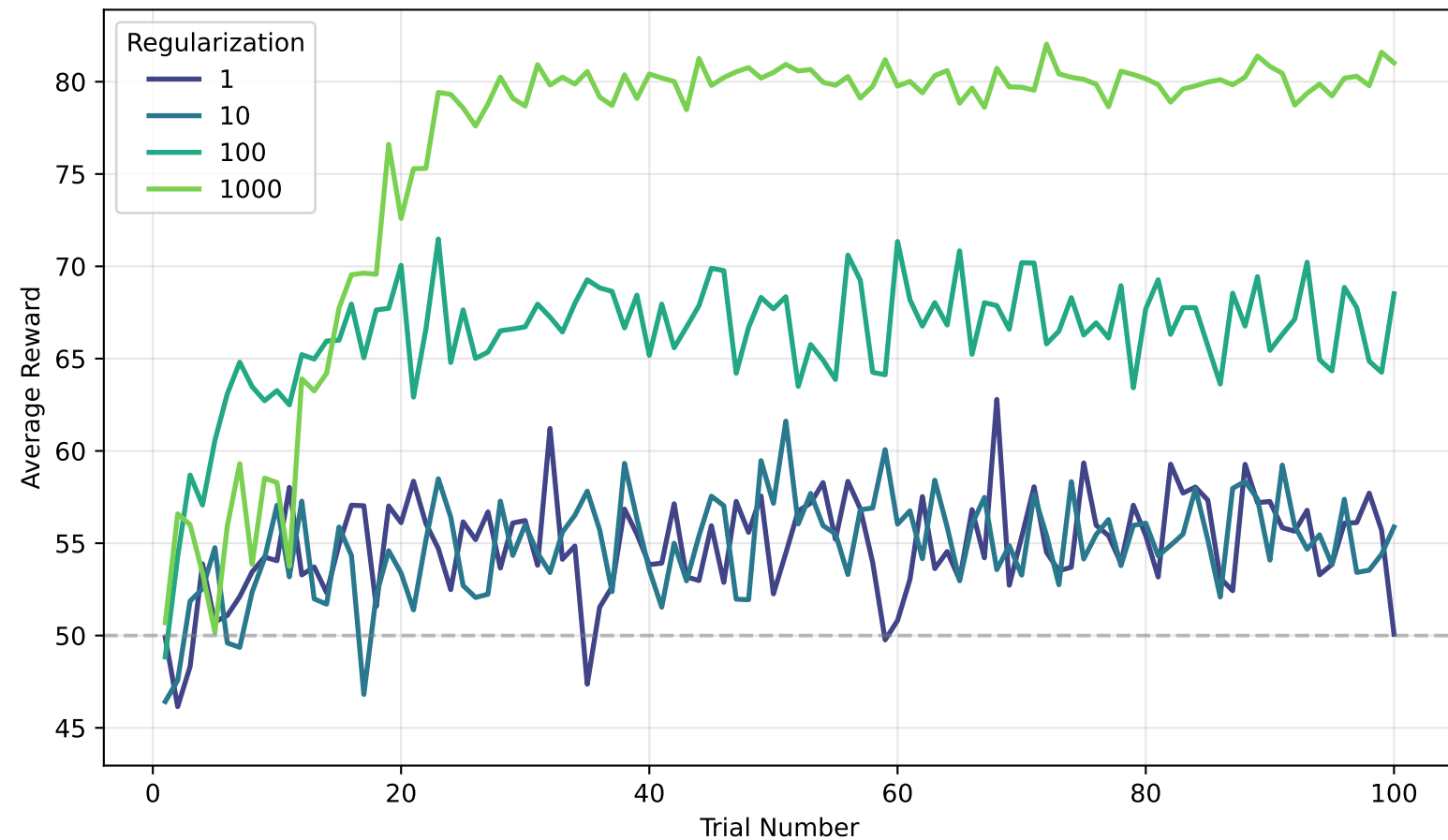
Linear UCB Performance
