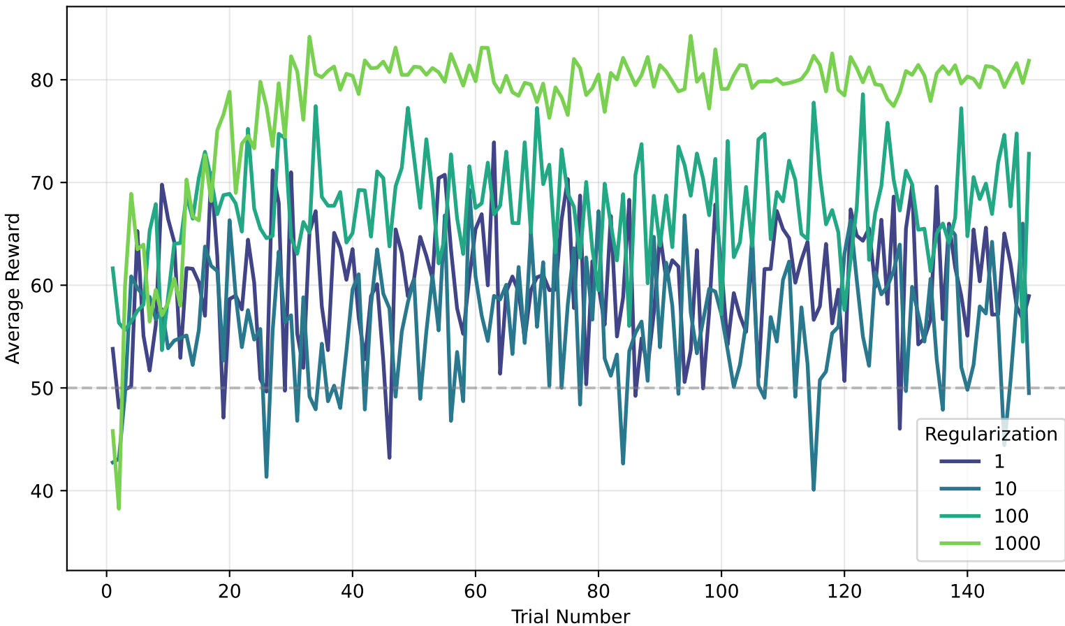
Linear UCB Performance
