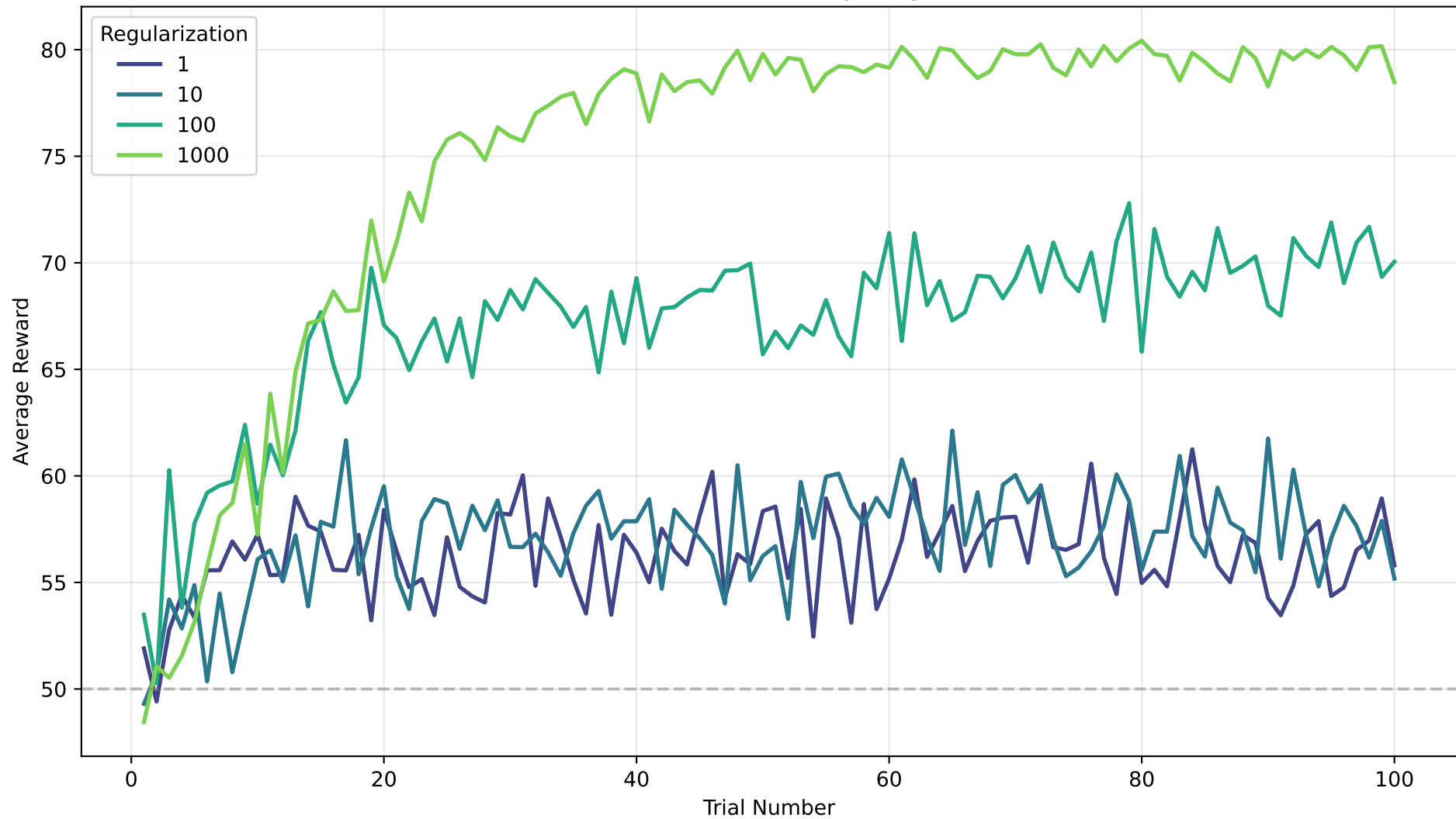
Linear UCB Performance by Regularization
