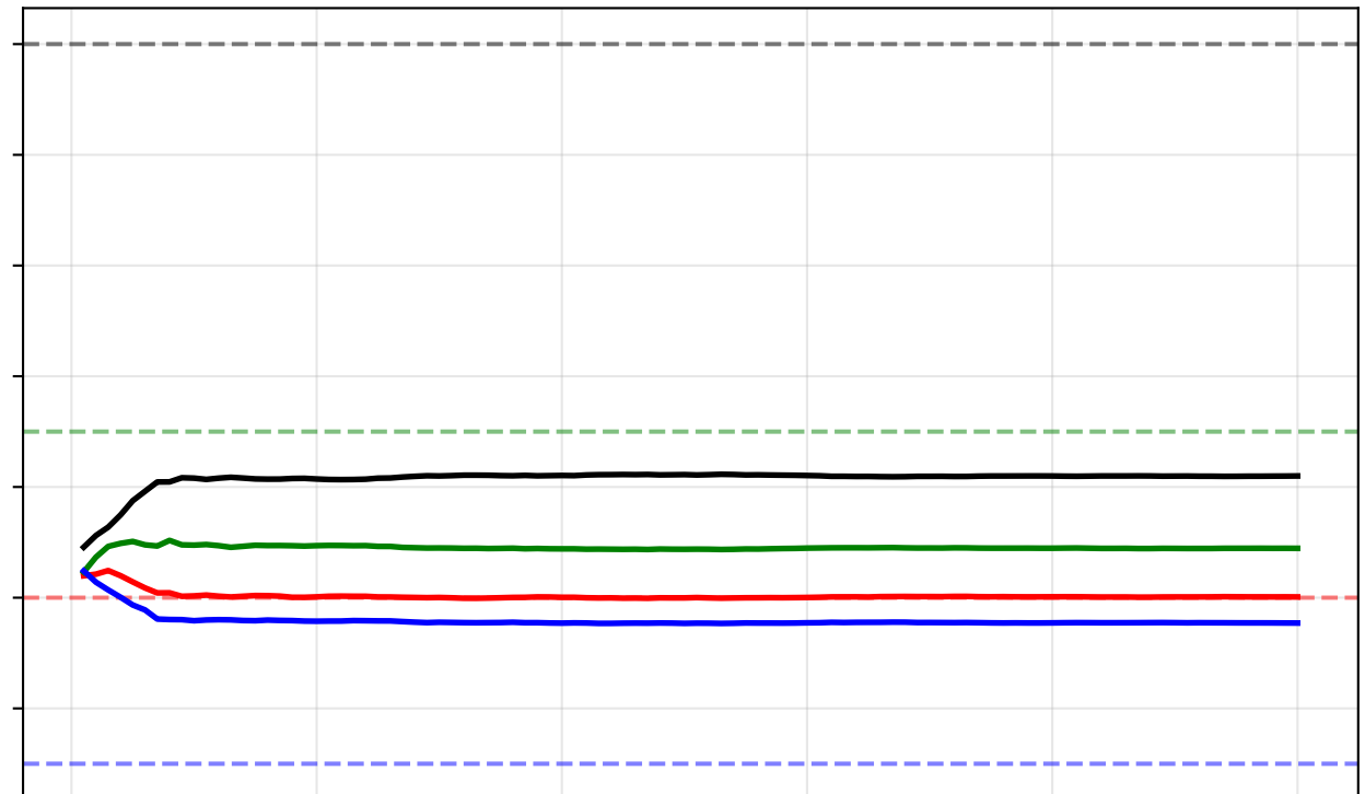
Planet B Weights Evolution
