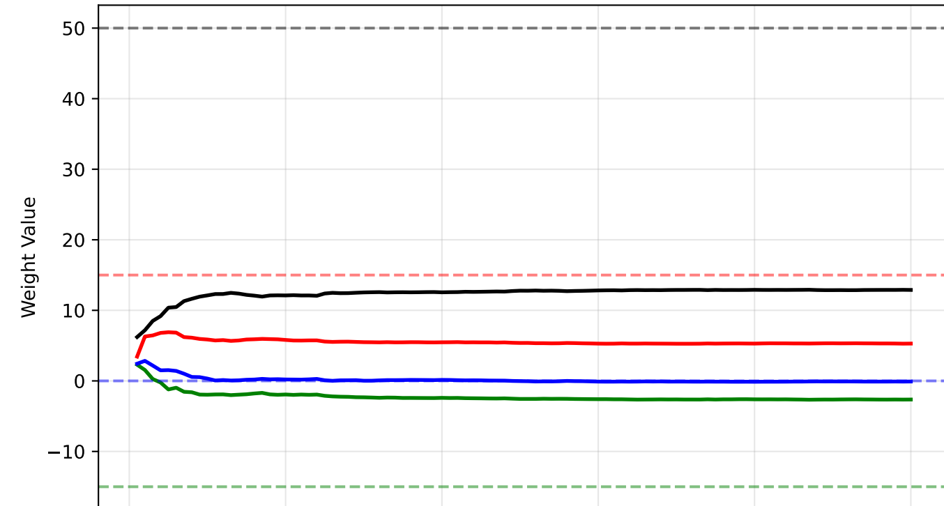
Planet A Weights Evolution
