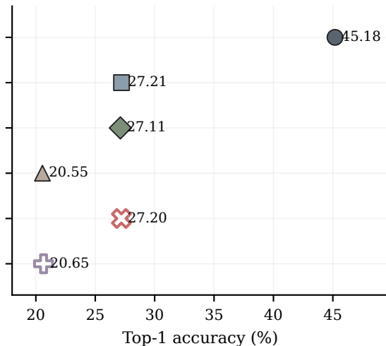
Accuracy boundary
