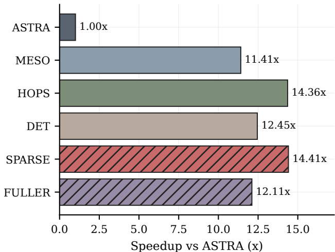
Runtime readiness
