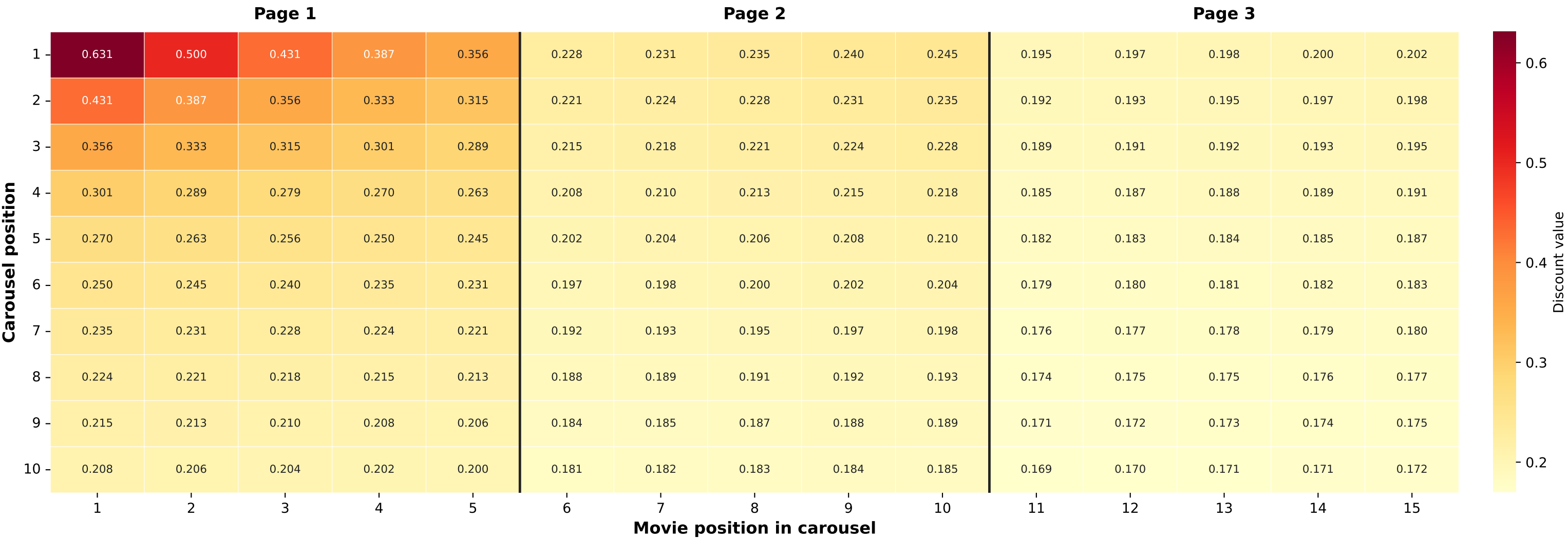
Mirrored F-Pattern with Additive Swipe Penalty
