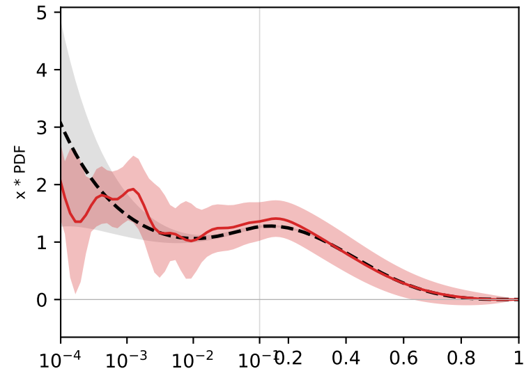
v3 (isovector)
