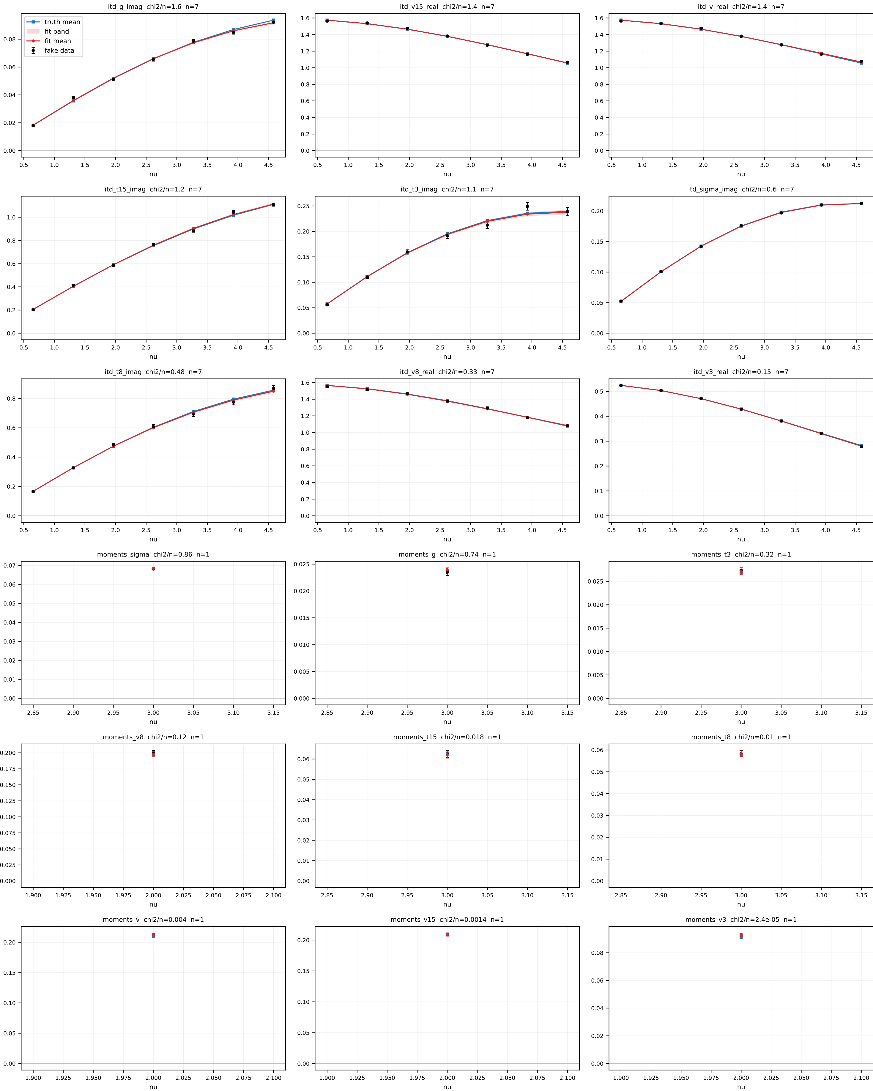
Closure observable reproduction: truthQ_1 (Q=1.0 GeV), mode=lattice; panels sorted by chi2
