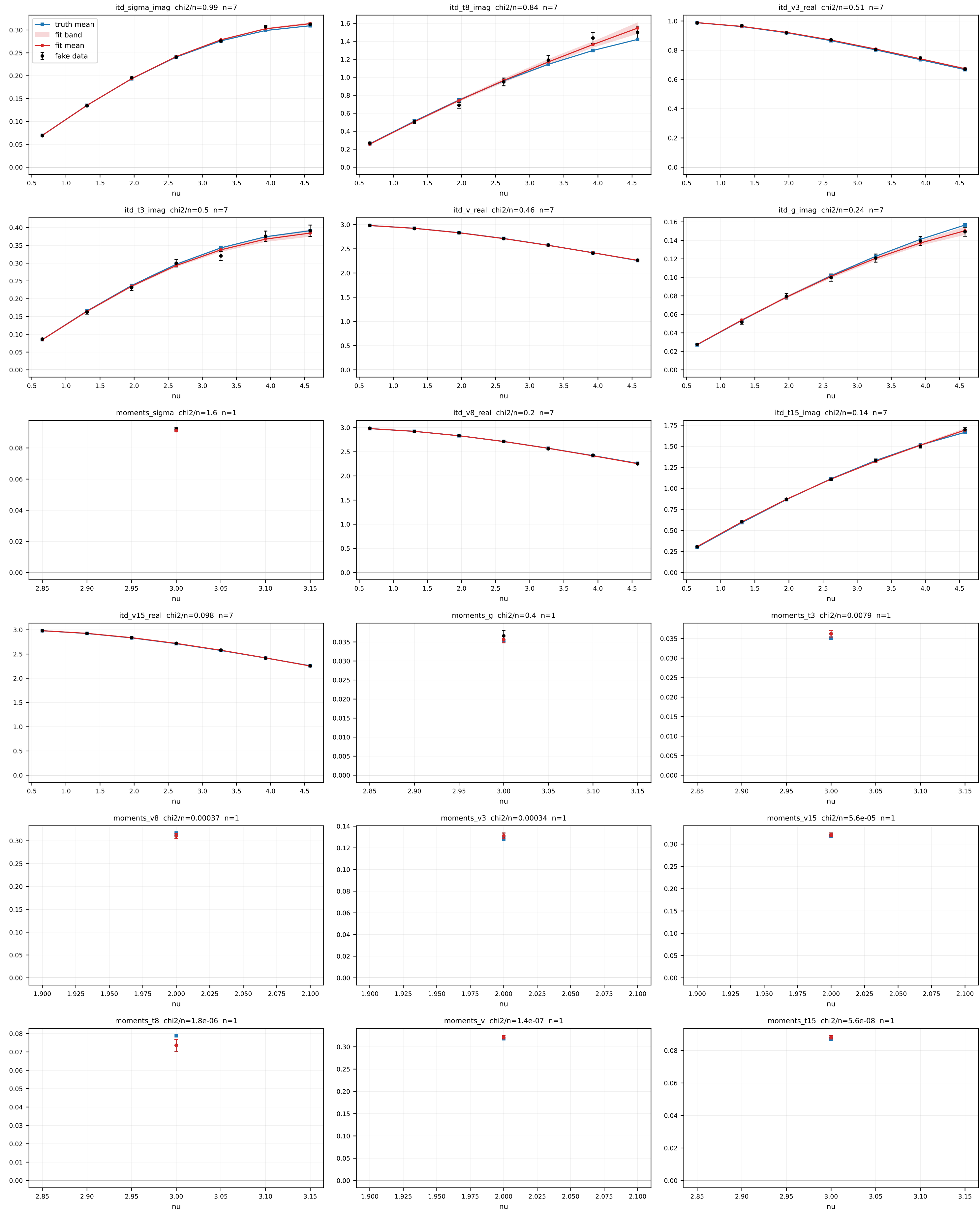
Closure observable reproduction: truthQ_5 (Q=5.0 GeV), mode=lattice; panels sorted by chi2
