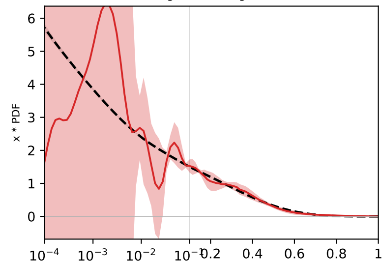
v3 (isovector)
