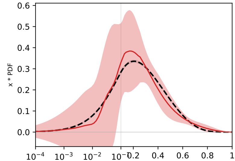
v15 (charm (V15))
