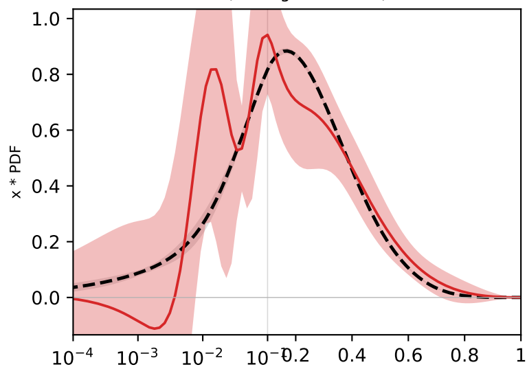
v (isosinglet valence)
