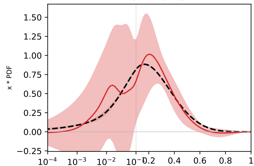
v15 (charm (V15))
