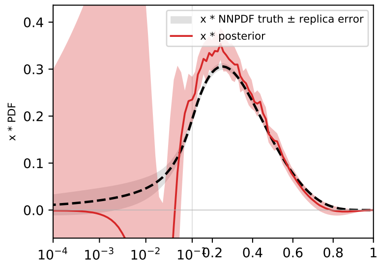
t15 (charm (T15))
