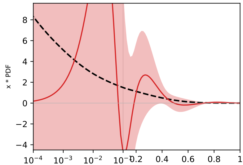
v3 (isovector)
