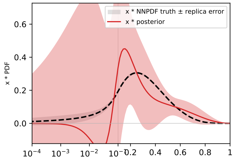
t15 (charm (T15))
