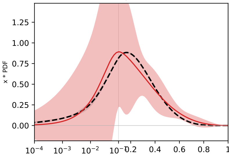
v (isosinglet valence)
