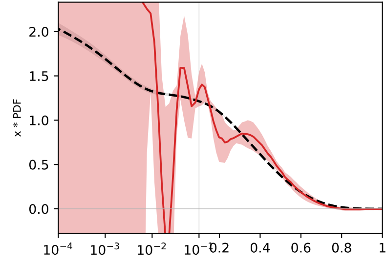
v3 (isovector)
