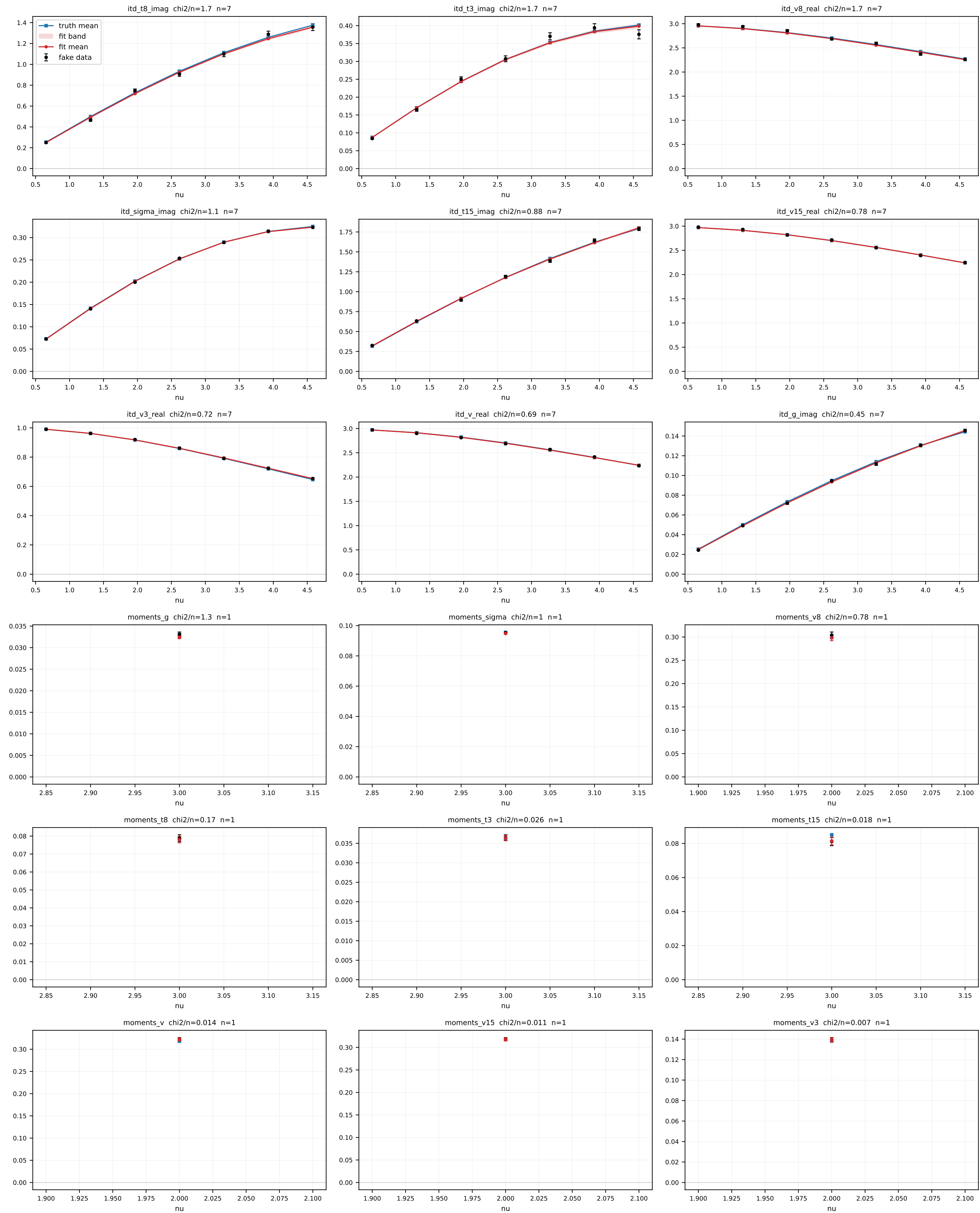
Closure observable reproduction: truthQ_4 (Q=4.0 GeV), mode=lattice; panels sorted by chi2
