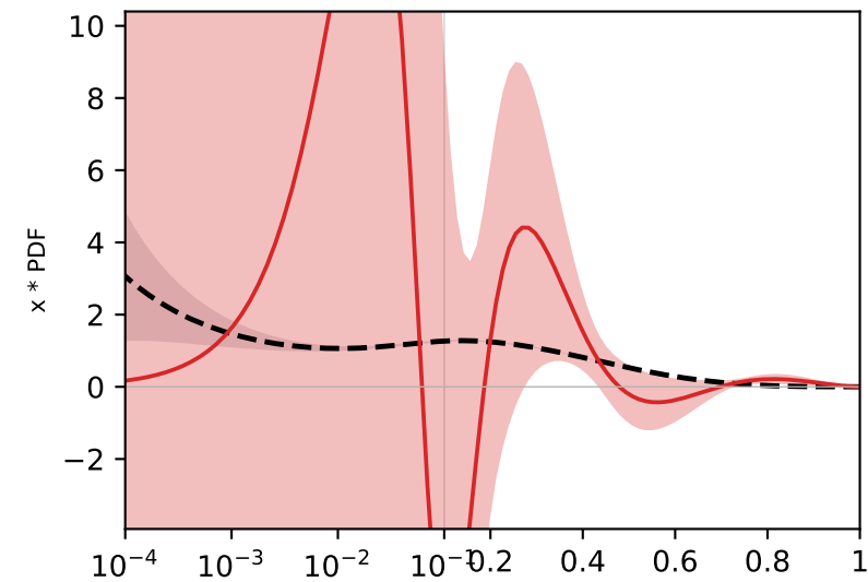
v3 (isovector)
