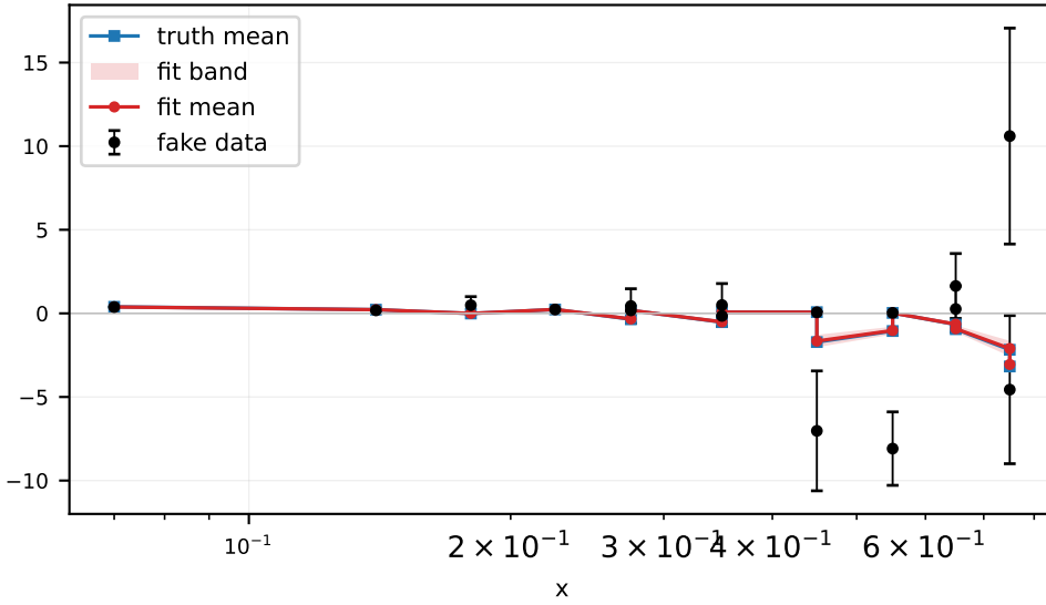
hera_cc_ep_318_sigmar chi2/n=0.72 n=16
