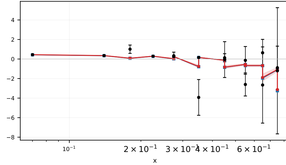
hera_cc_em_318_sigmar chi2/n=0.71 n=16
