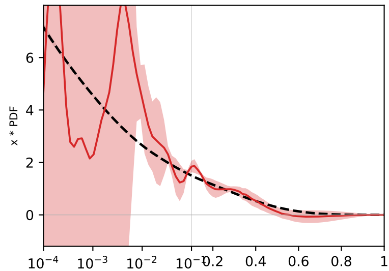
v3 (isovector)
