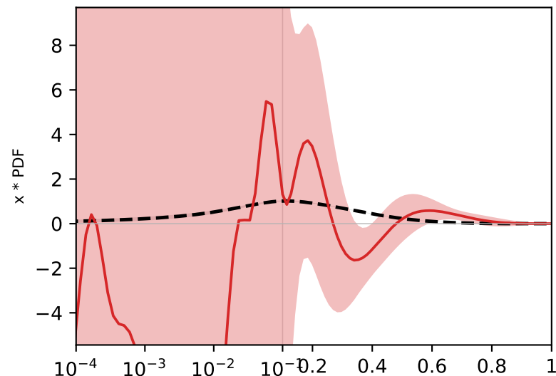
t8 (strange (T8))
