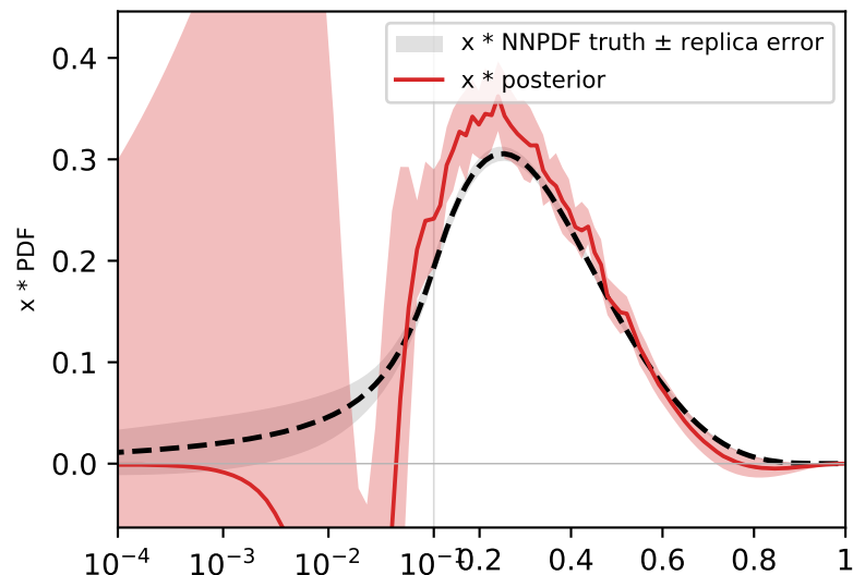
t3 (isovector)
