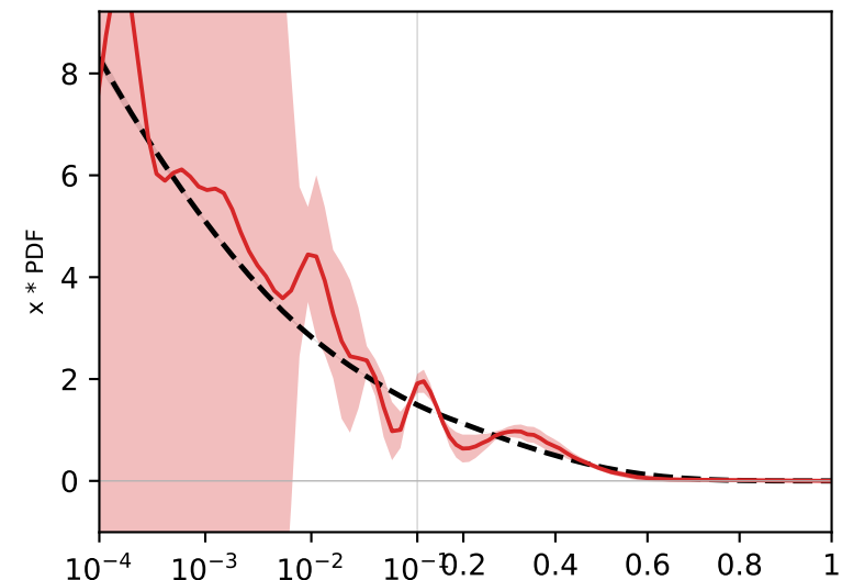
sigma (isosinglet)
