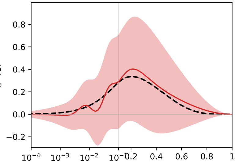
v15 (charm (V15))
