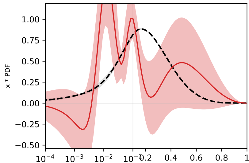
v (isosinglet valence)
