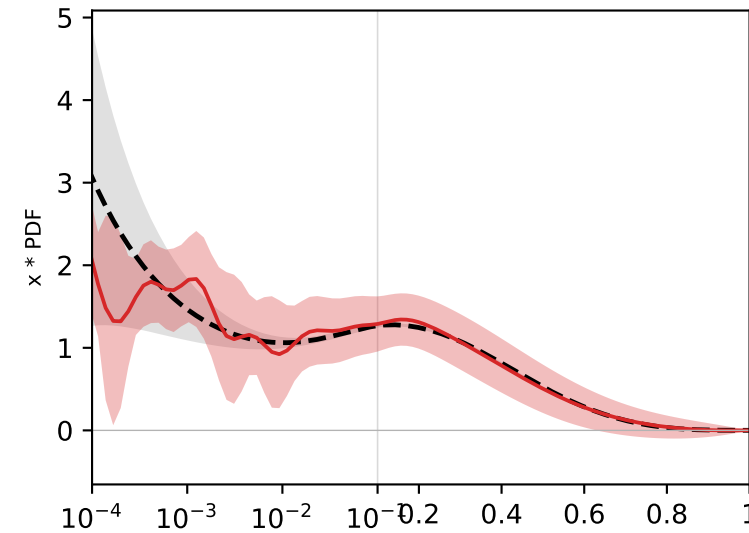
v3 (isovector)
