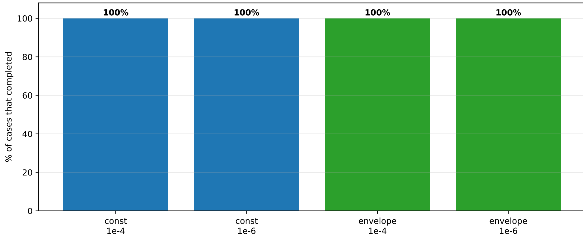
Fits that ran at all, by prior form and constraint strength (72 cases each: 2 truths x 6 scales x 6 modes)
