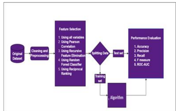
Fig 2. Applying the MLP Method
