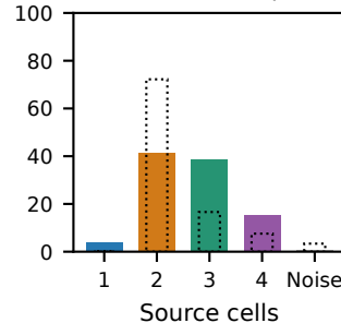
h PC1 source composition
