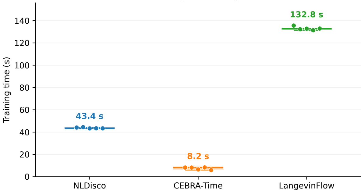
LVM training time comparison
