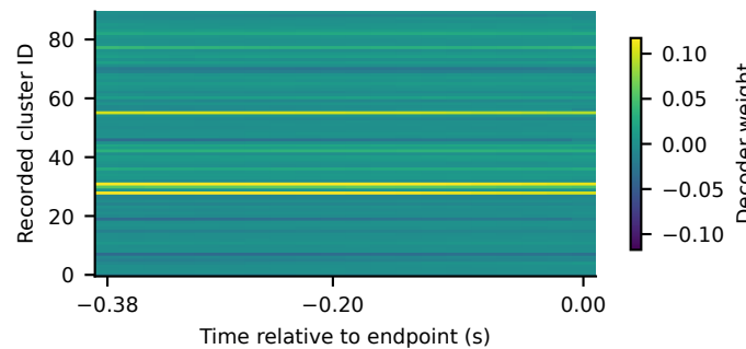
Highest centroid-speed quintile: 109 Temporal decoder weights
