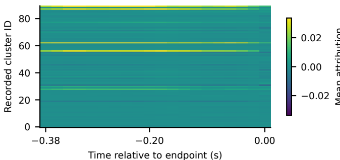
Radially outward movement: 10 Encoder attribution
