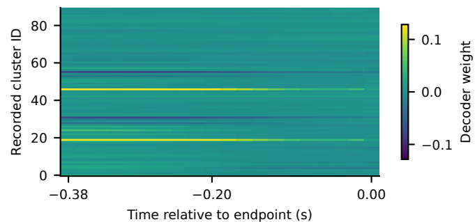
Smaller area near the patch: 107 Temporal decoder weights
