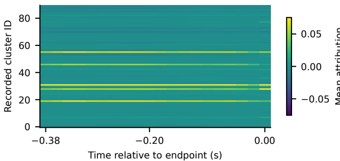
Highest centroid-speed quintile: 109 Encoder attribution
