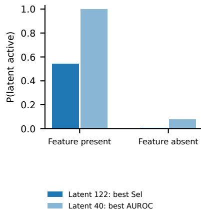
b Activation probability
