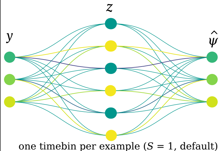
b SED reconstruction of neural activity
