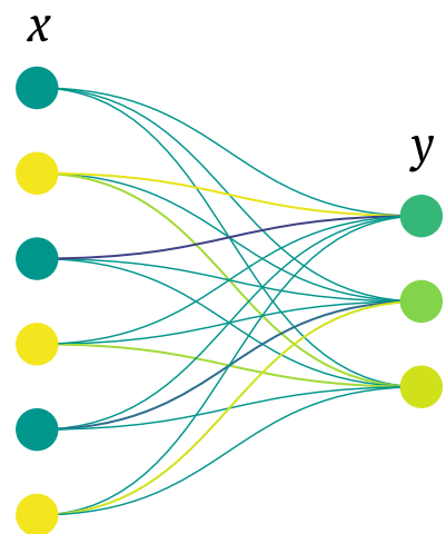
d Window SED: reconstructing a sequence of S timebins
