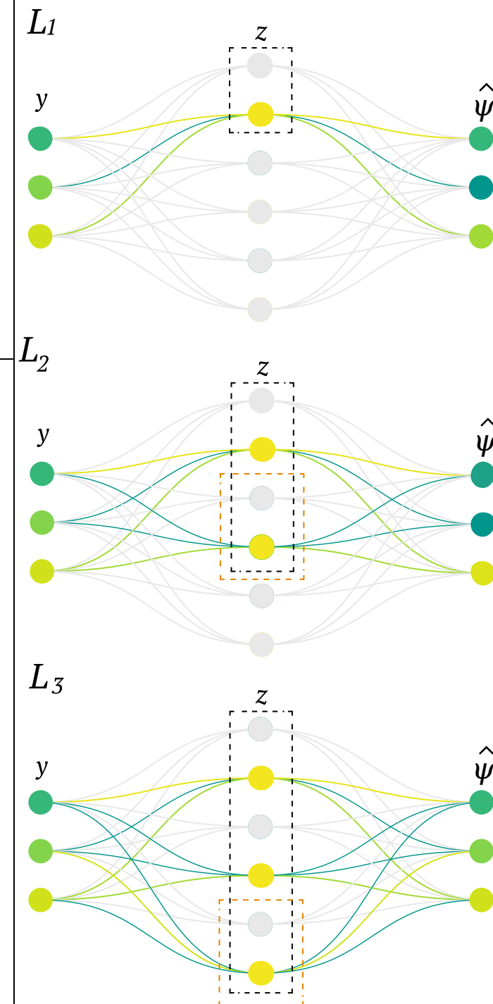
c Matryoshka SED reconstruction
