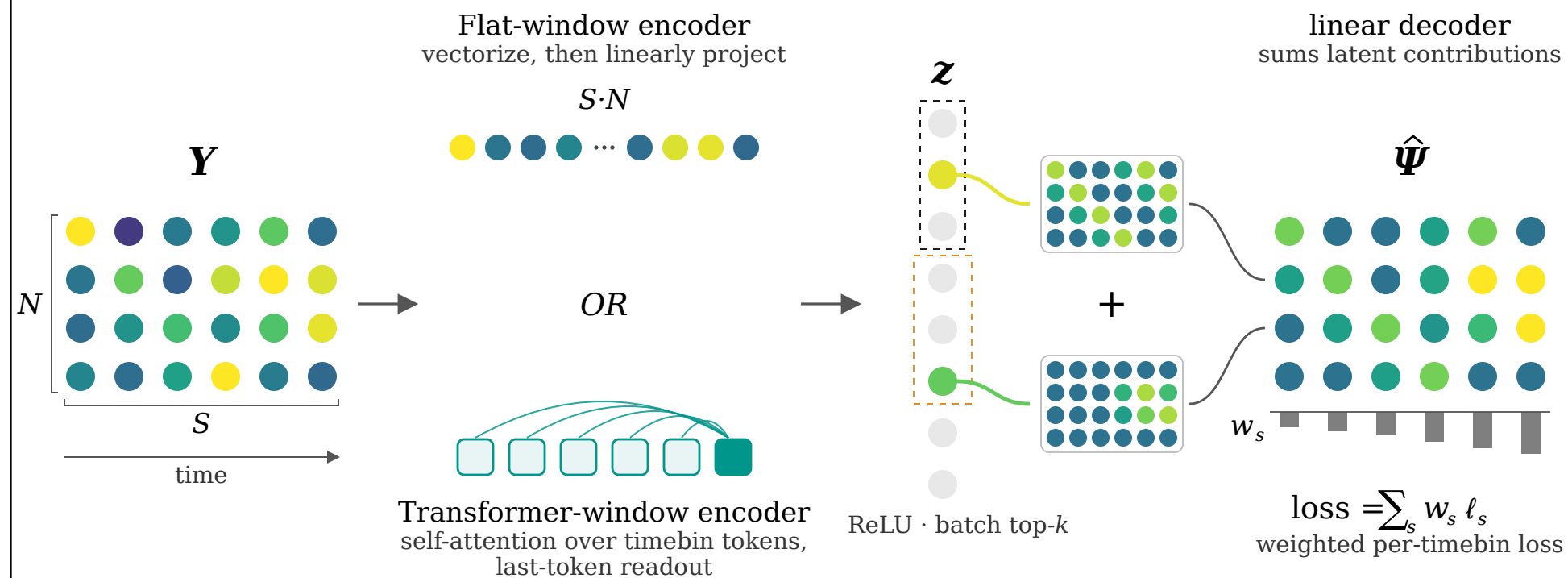
d Window SED: reconstructing a sequence of S timebins
