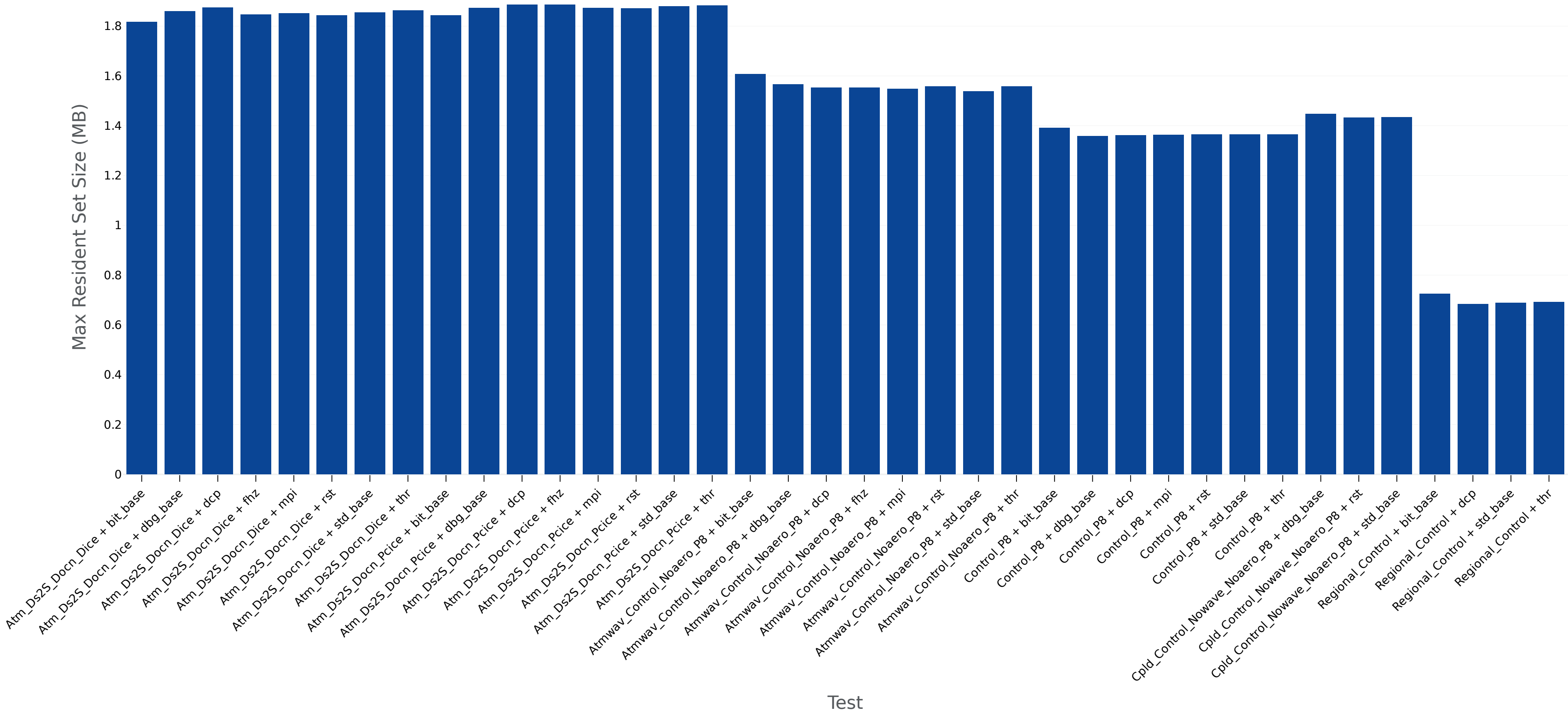
Operation Requirement Test Framework: Maximum Resident Size vs Test Performed on Hera
