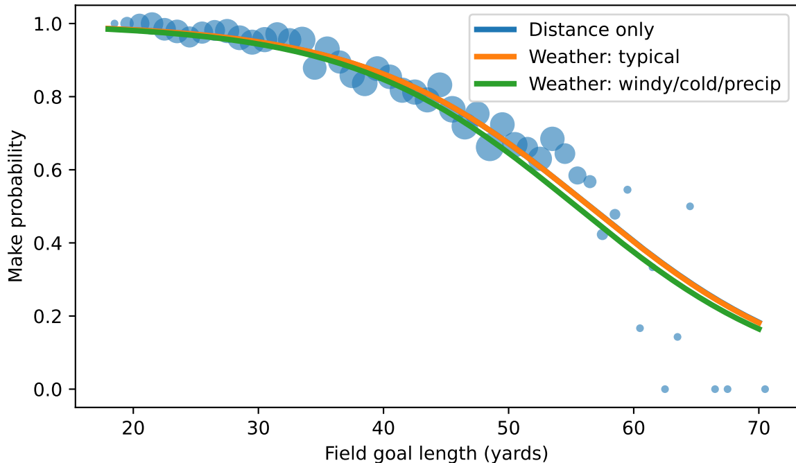
FG make probability vs distance (logit) with weather covariates
