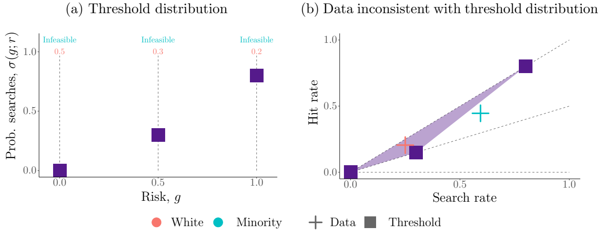
Figure 2: How search and hit rates are informative of thresholds
