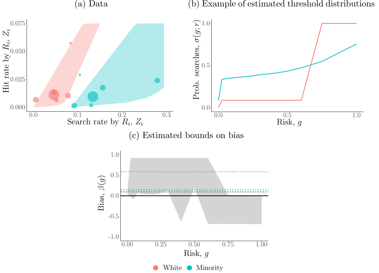
Figure 8: Example where bias is detected
