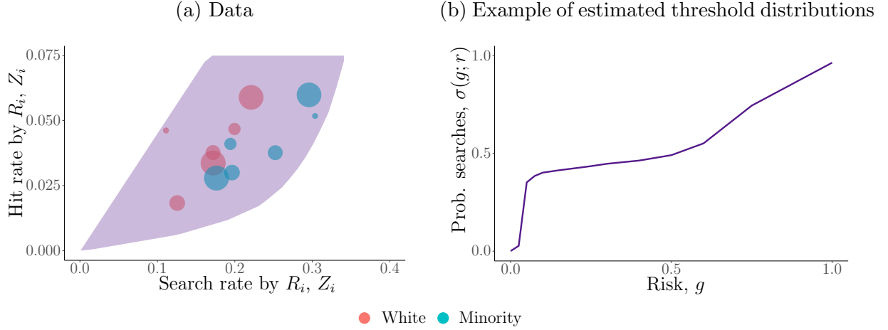
Figure 7: Example where bias is not detected
