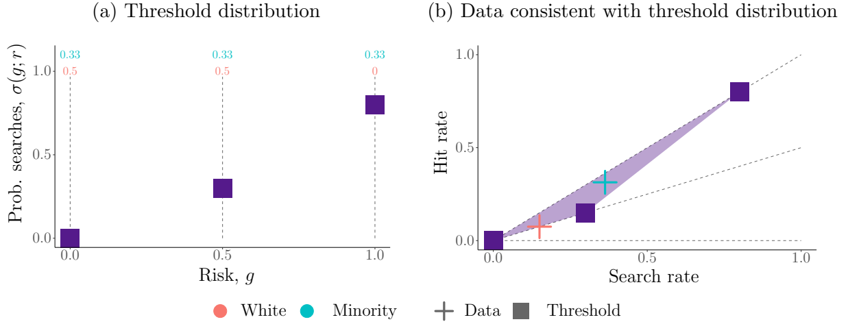
Figure 1: How search and hit rates are generated
