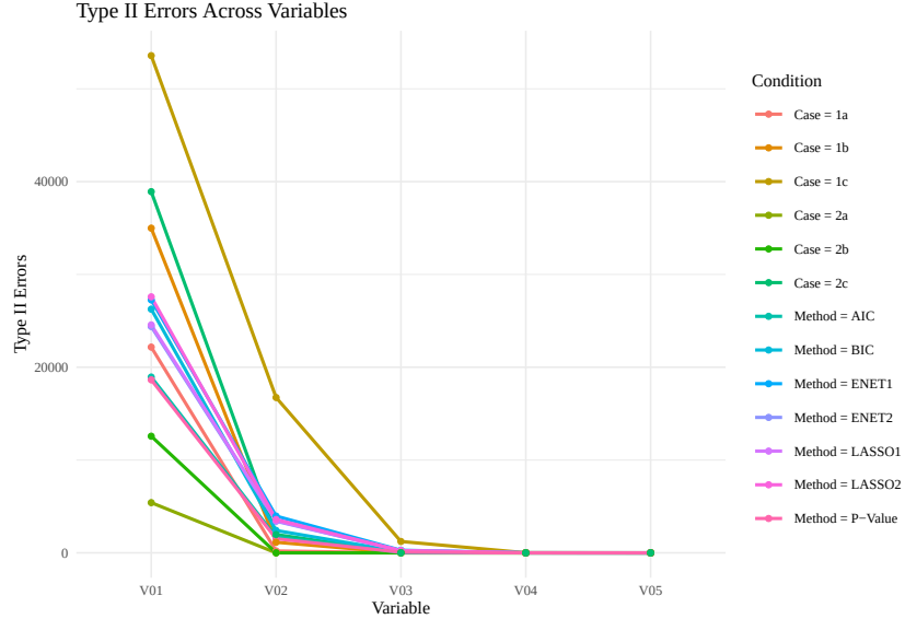
Figure 2: Type II error by magnitude of association, for methods and cases
