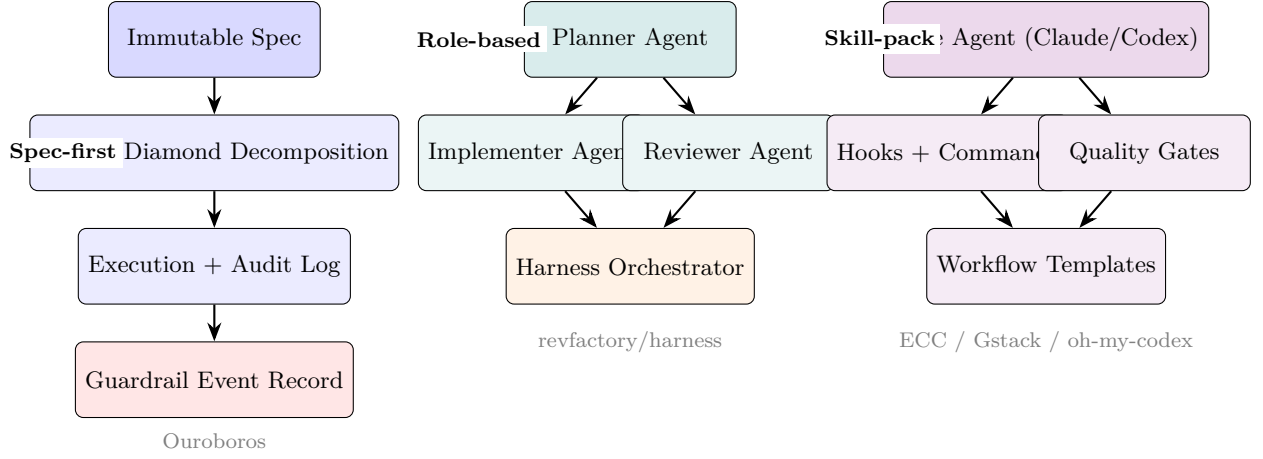
Figure 3: Three architectural patterns identified among evaluated harness tools. (a) Spec-first: constraints are crystallized into immutable specifications before execution, providing audit-grade traceability. (b) Role-based: work is decomposed across specialized agent roles with explicit responsibilities. (c) Skill-pack: existing agents are extended with hooks, commands, and quality gates.
