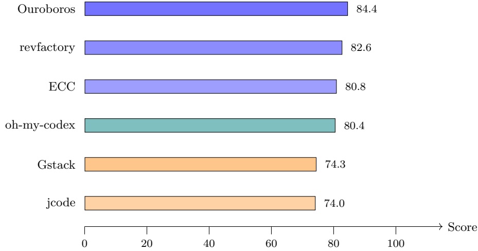
Figure 1: Normalized 100-point overall scores. The top four tools (blue/teal) form a cluster above 80, while the bottom two (orange) score below 75, driven primarily by T5 guardrail performance.
