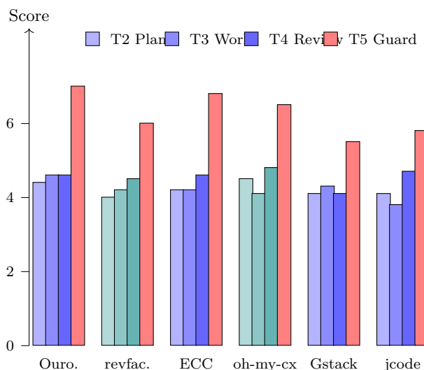
Figure 2: Per-task scores by tool. Blue/teal bars (T2–T4) cluster tightly across tools; red bars (T5 Guardrail) show the widest spread, confirming guardrail enforcement as the primary differentiator.
