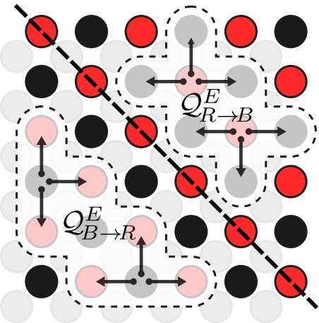
(a) Microscopic QCA bath
