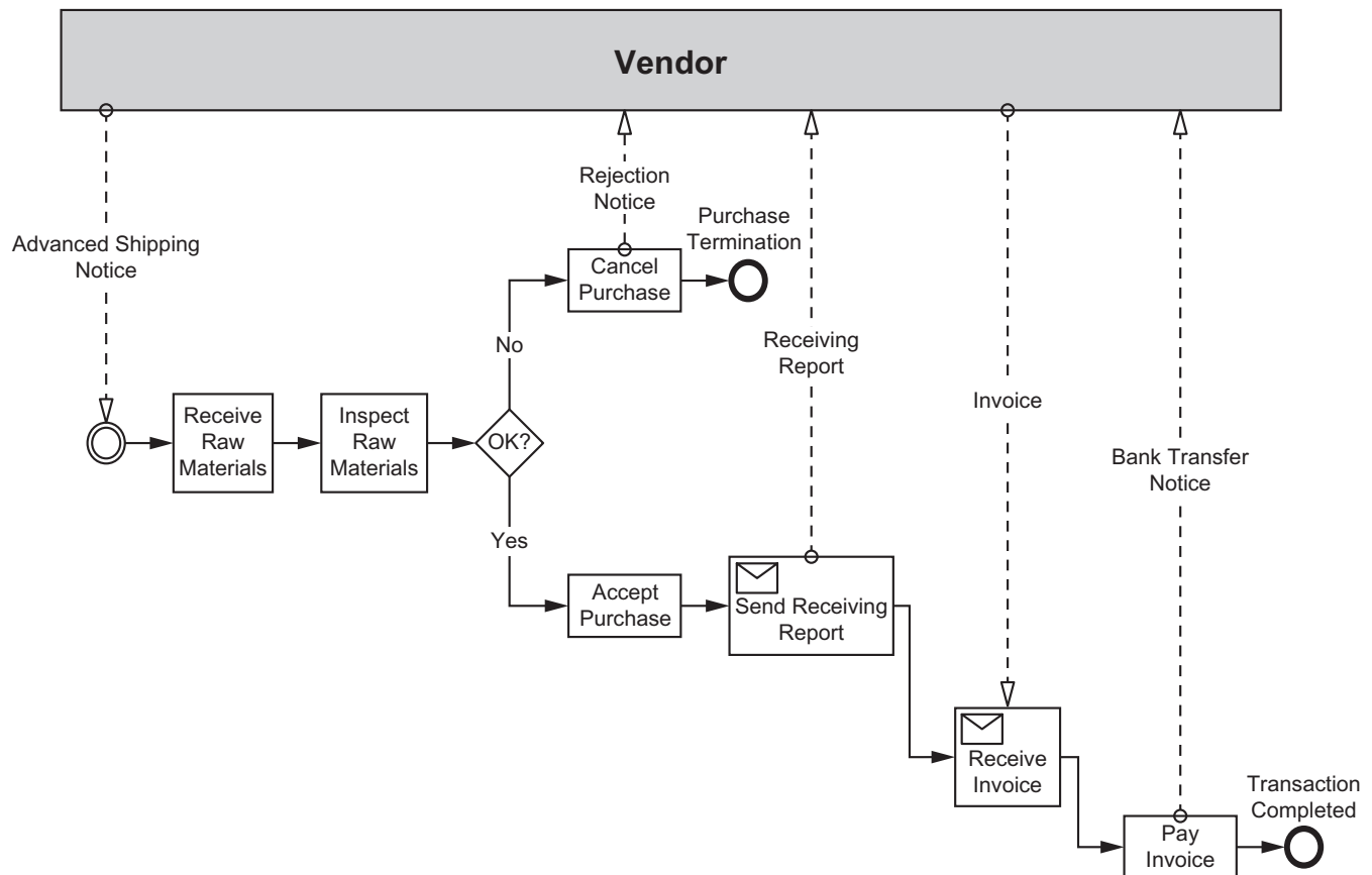
FIGURE 2-4 BPMN Workflow for Raw Material Acquisition and Payment
