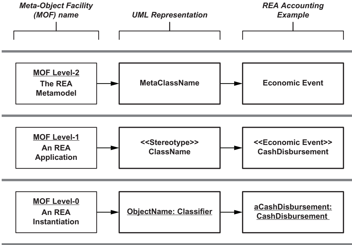
FIGURE 1-6 Shorthand Use for the Meta-Object Facility (MOF)
