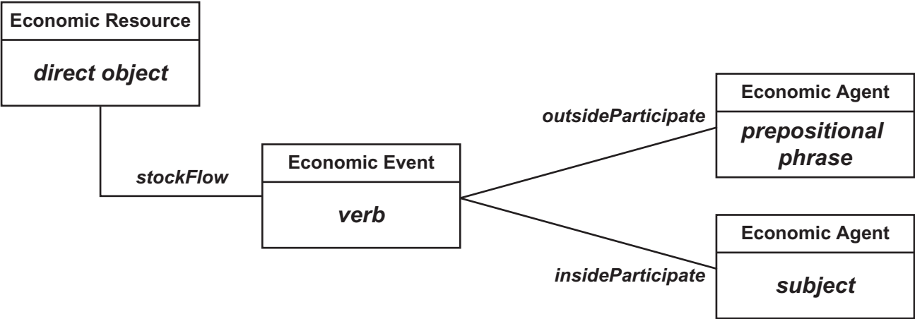
(a) – Sentence Translation of the REA Metamodel
