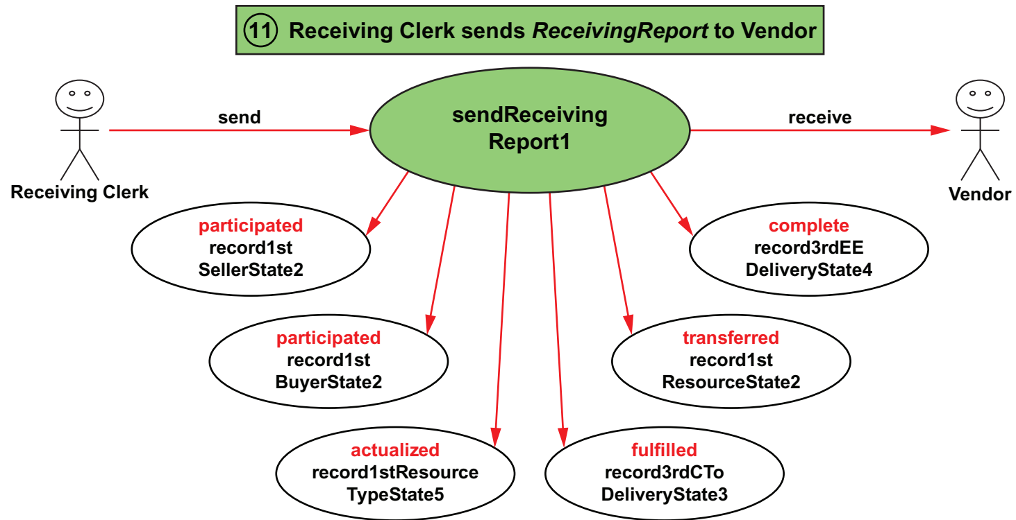
FIGURE 6-5 Effect of Business Event on Object States (Source: Horiuchi and McCarthy 2011 )
