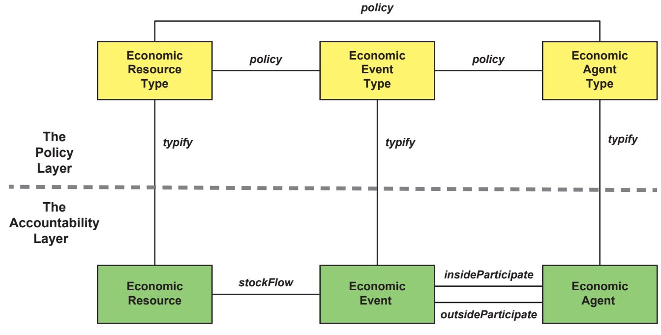
FIGURE 3-6 REA Accountability/Policy Layer Interaction (M2)
