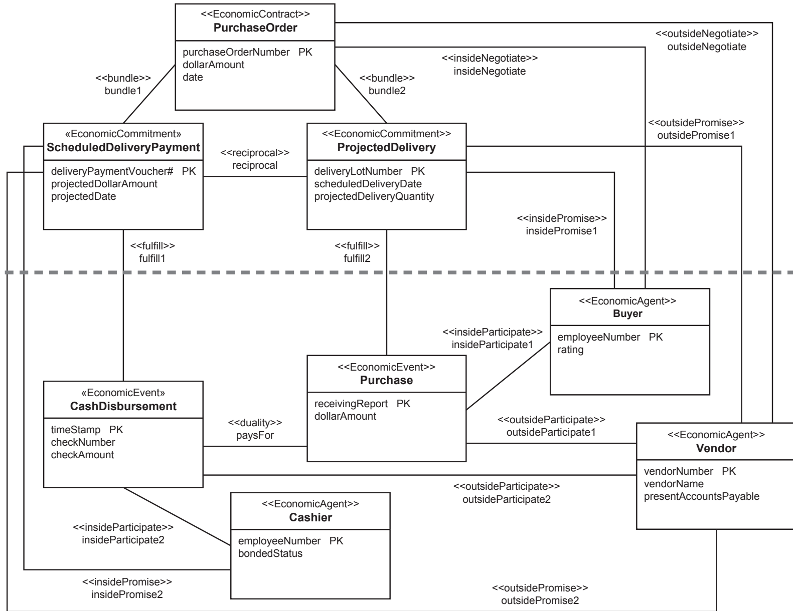
FIGURE 3-10 REA Accountability/Scheduling Layers with Agents (M1)
