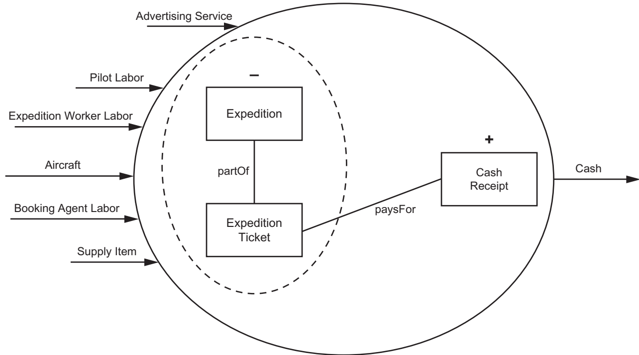
FIGURE 4-12 AAE Business Process with Meronymic Expansion of an Event Slot
