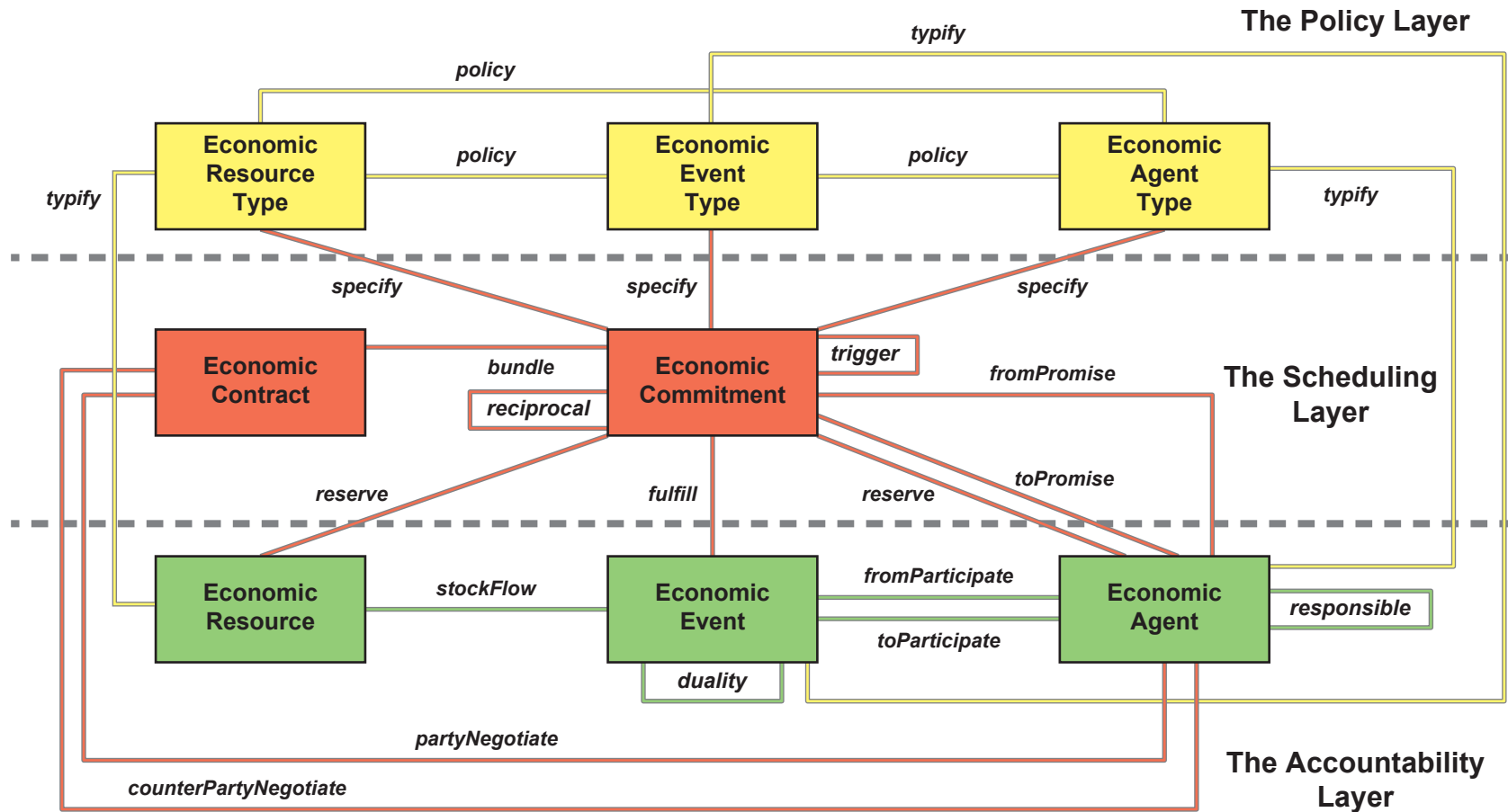
FIGURE 5-8 The REA Metamodel (Independent View at MOF M2)
