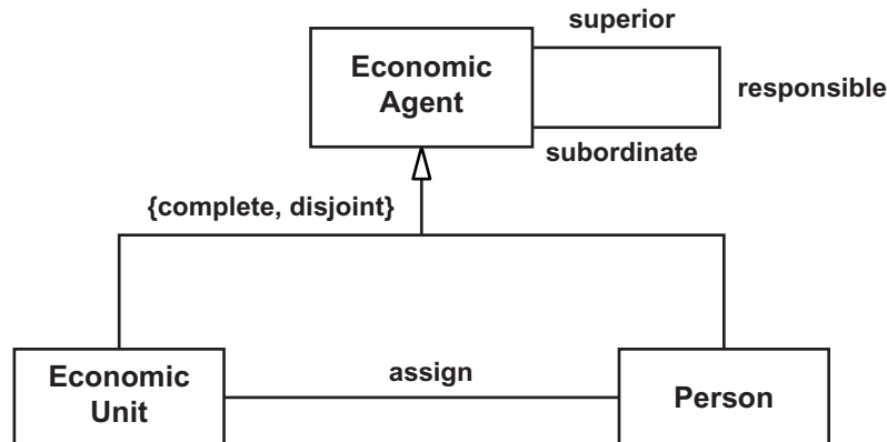
FIGURE 1-9 Agent Generalization Hierarchy
