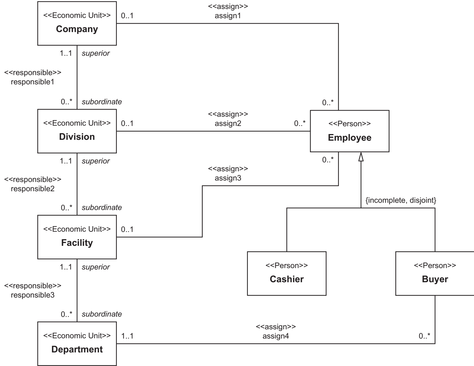
FIGURE 1-14 An M1 example of REA Agent Subtypes with Organizational Economic Units
