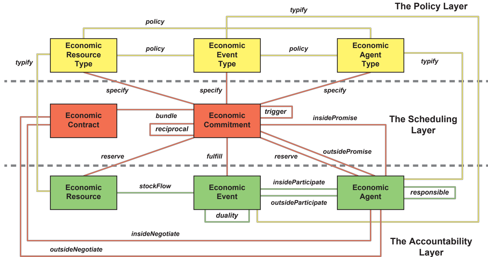
FIGURE 3-16 The REA Metamodel (M2) for All Temporal Layers
