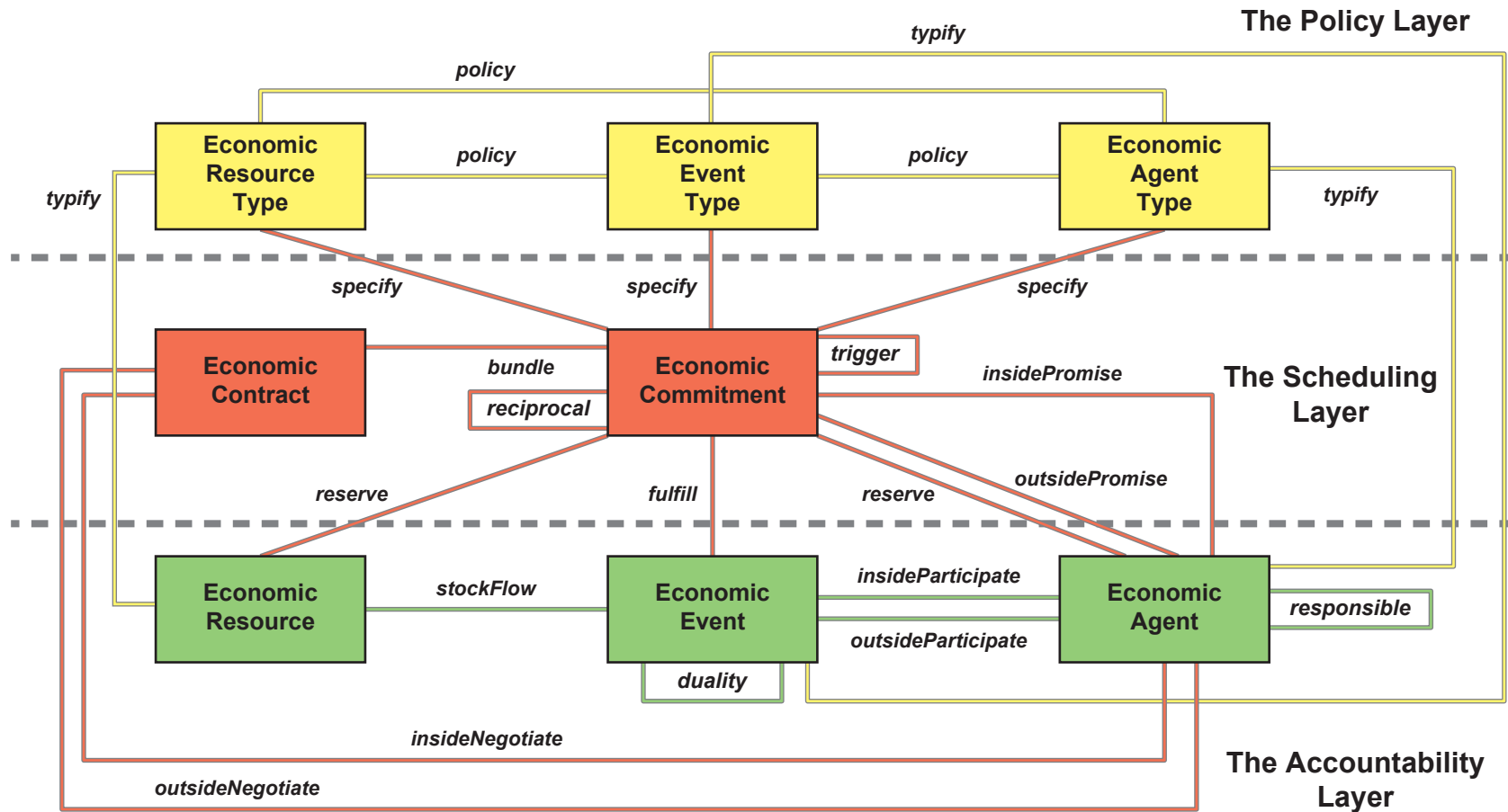
FIGURE 5-5 The REA Metamodel (Trading Partner View at MOF M2)
