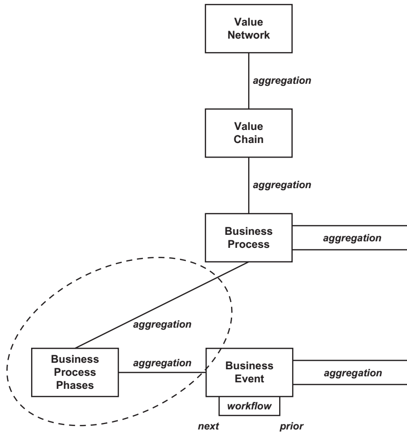
FIGURE 4-15 Adding Process Phases to REA Granularity Levels
