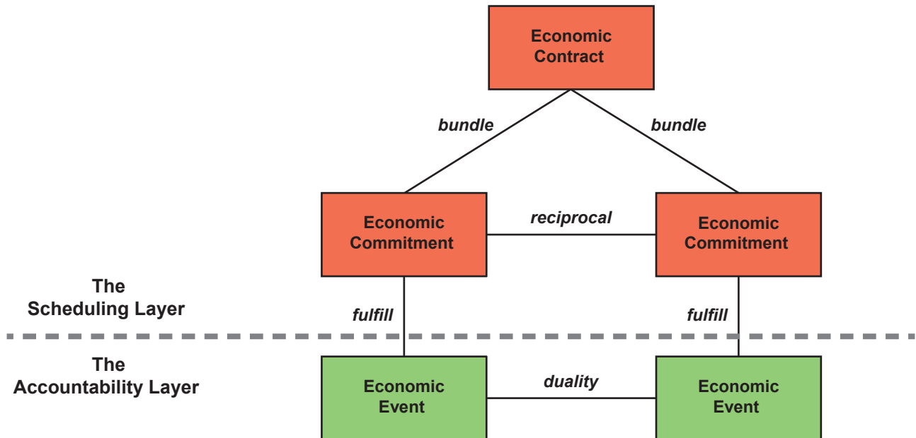
FIGURE 3-8 REA Accountability/Scheduling Layer Interaction with Symmetrical Event and Commitment Images -- M2
