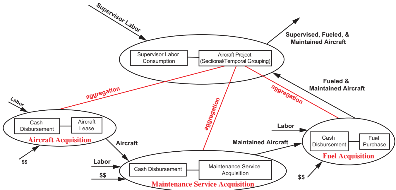
FIGURE 6-18 Process Hierarchy Aggregation for Supervisor Labor Input
