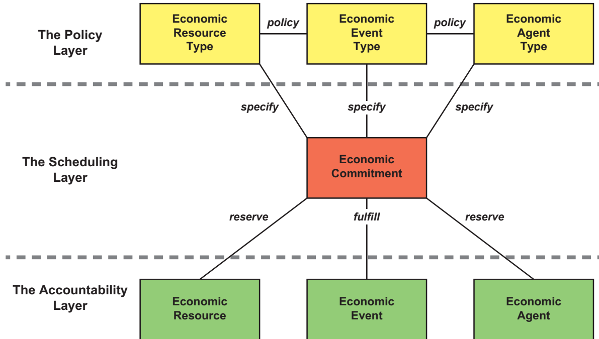
FIGURE 3-15 REA Accountability/Scheduling/Policy Specification and Reservation (M2)
