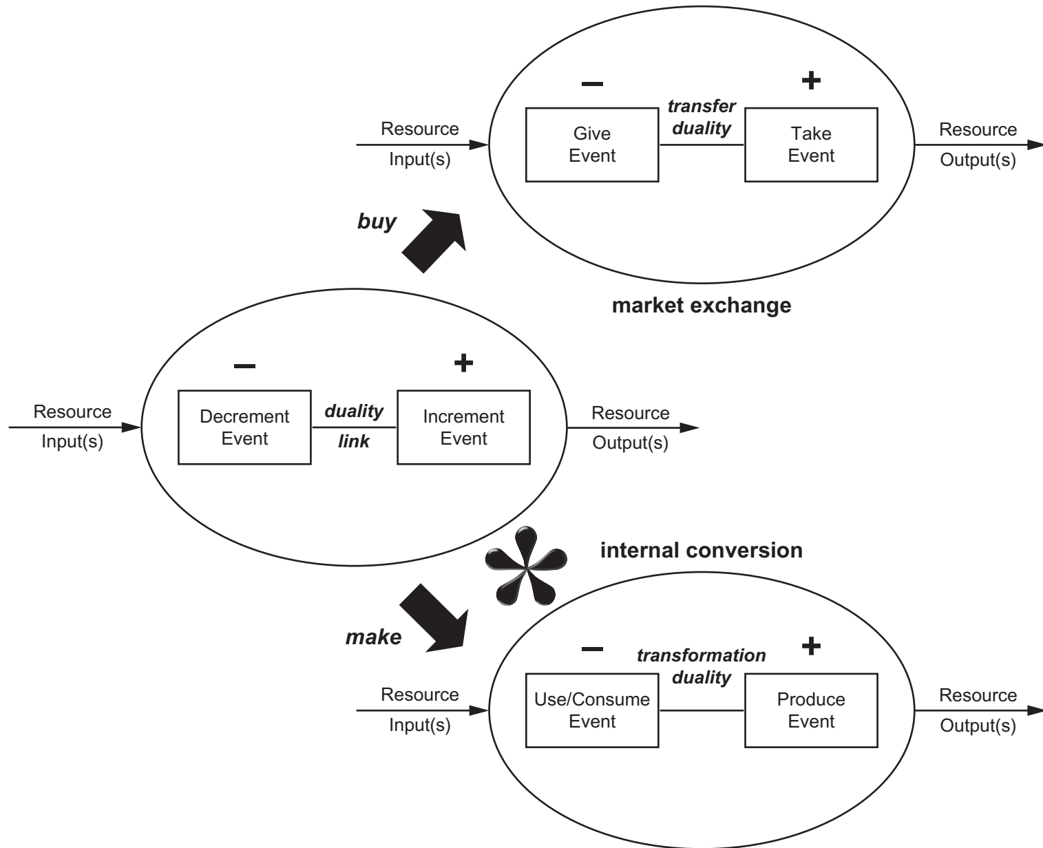
FIGURE 4-23 REA Duality Types: Buy (Transfer) vs. Make (Transformation)
