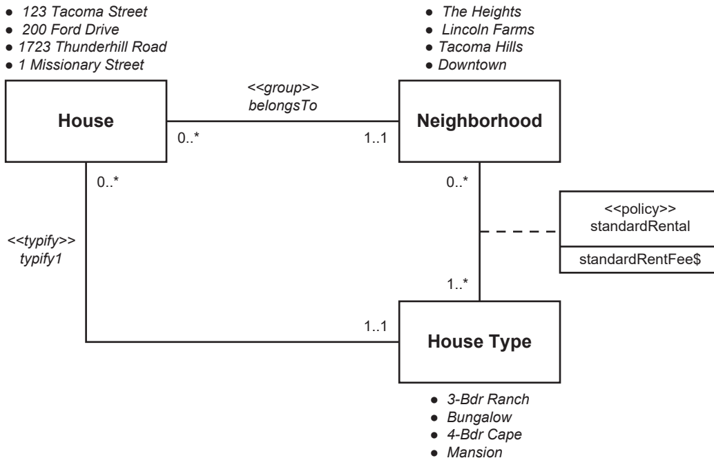
FIGURE 3-4 REA Policy Layer with Typification and Grouping
