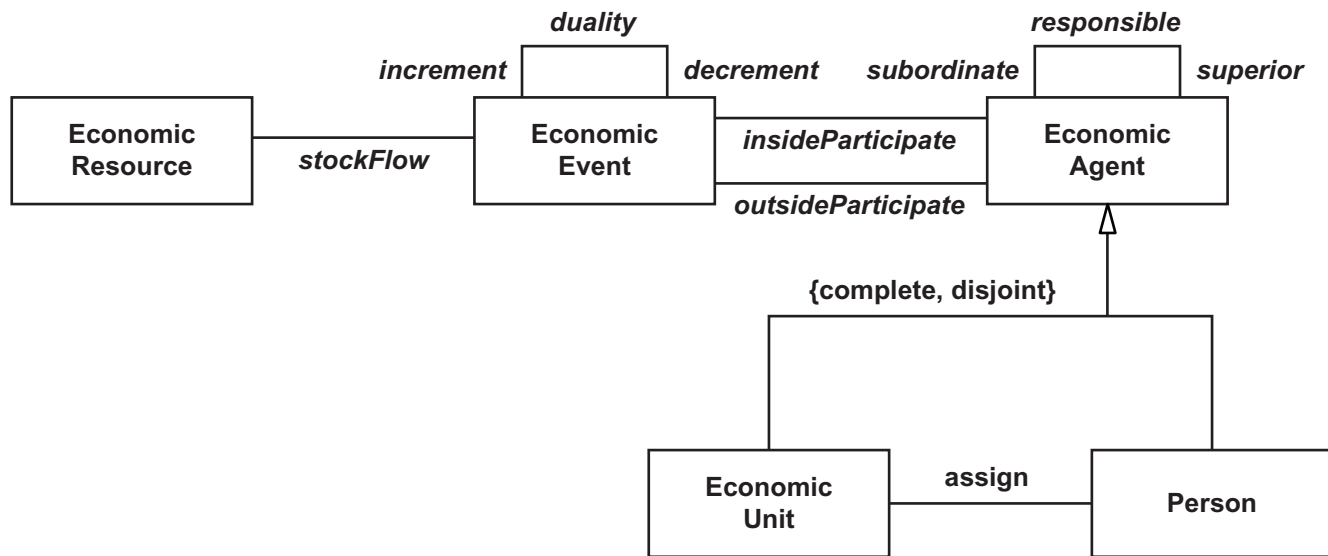
FIGURE 1-10 The REA Metamodel with Agent Generalization
