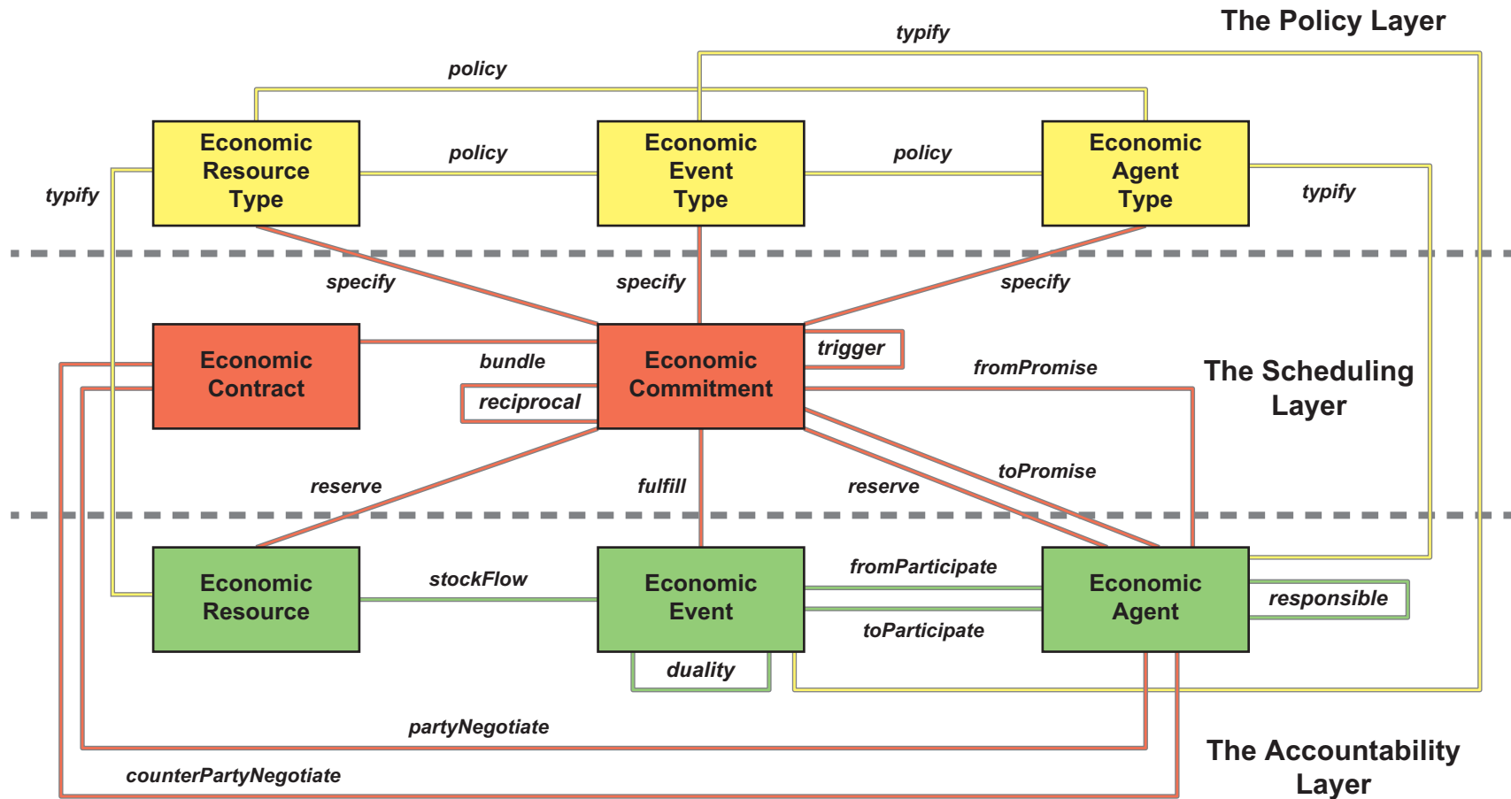
FIGURE 6-22 The REA Metamodel (Independent View)
