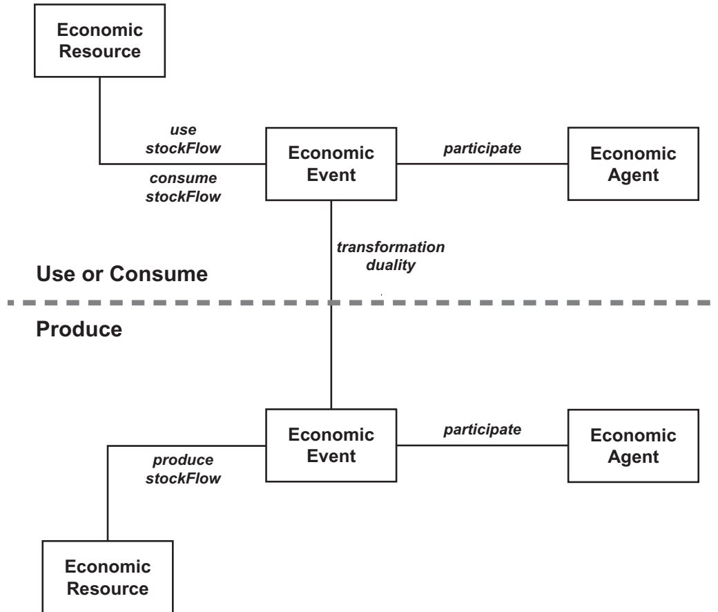
FIGURE 4-24 Accountability Pattern for Internal Conversion
