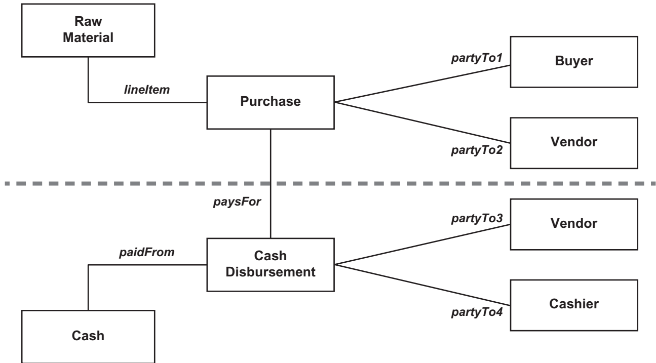
FIGURE 1-4 Class Diagram for Acquisition Business Process
