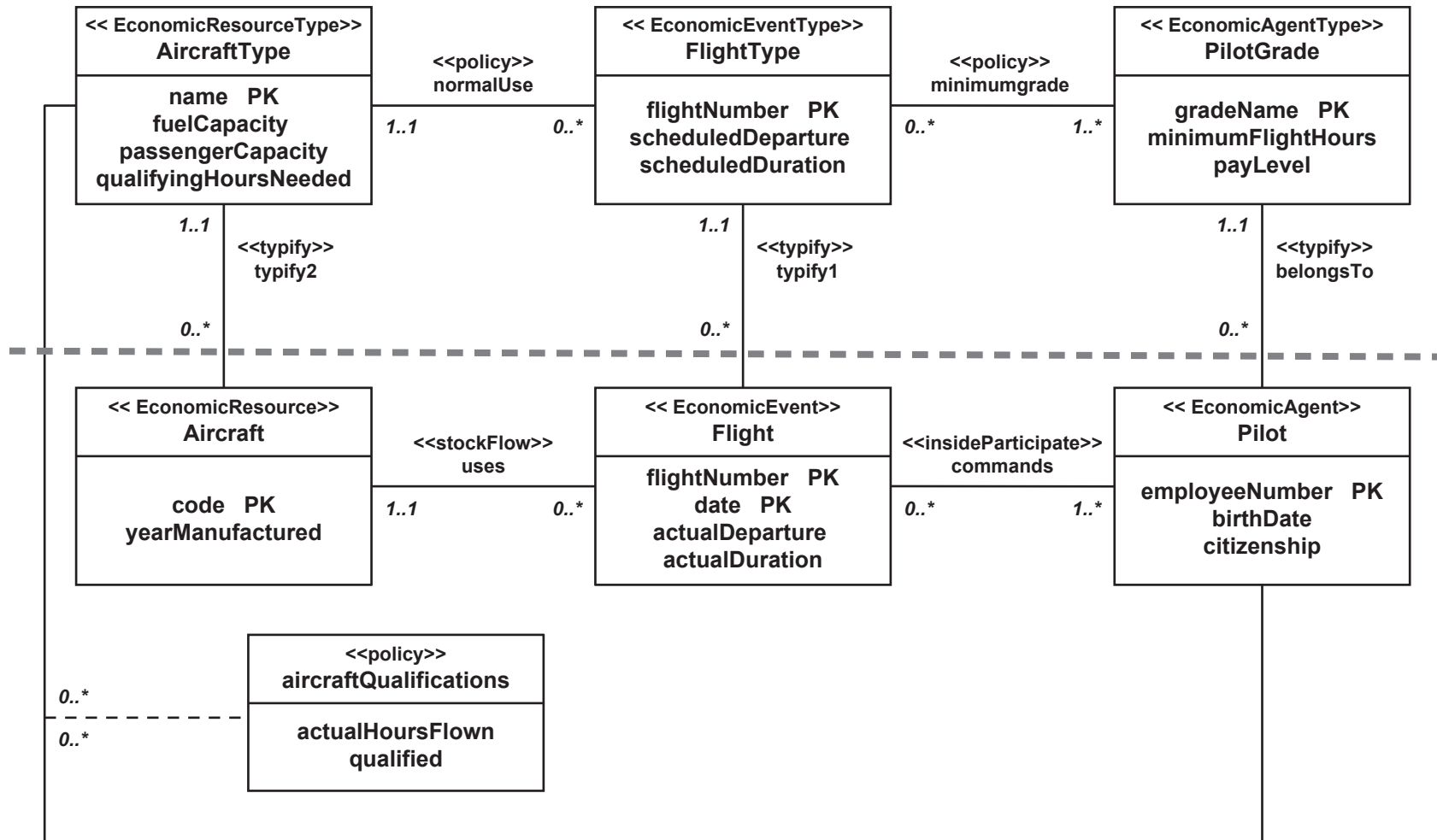
FIGURE 3-7 REA Accountability/Policy Layer Interaction (M1)
