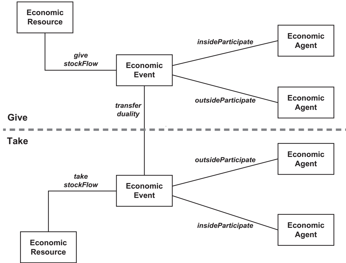
FIGURE 4-14 Accountability Pattern for Market Exchange
