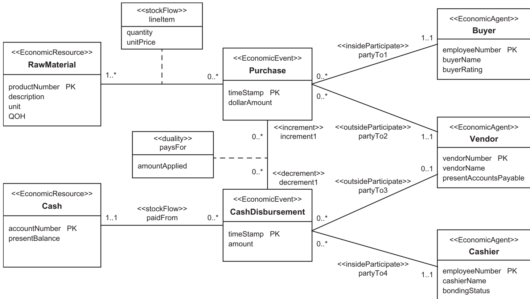
FIGURE 1-8 M1 Class Diagram for Acquisition Process (an REA Application) with Attributes, Multiplicities, and Stereotypes
