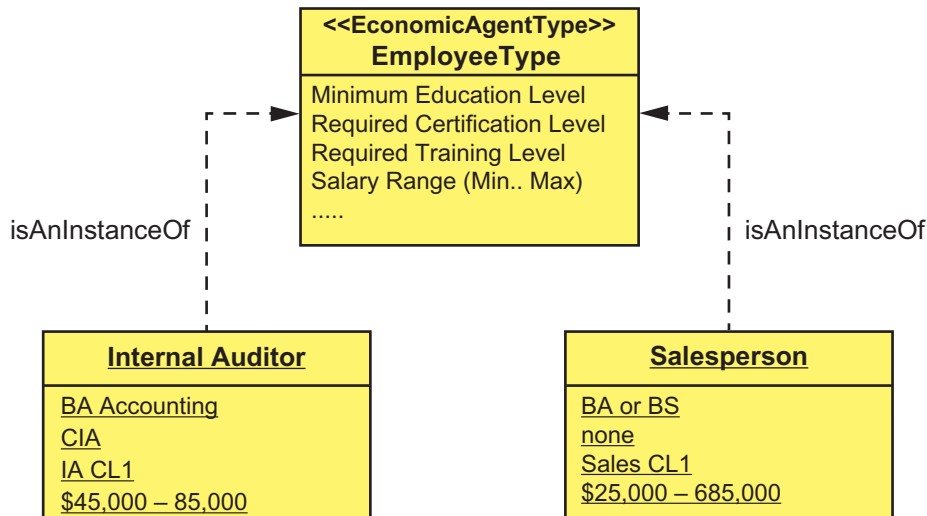
FIGURE 6-20 Two Instances of Employee Type
