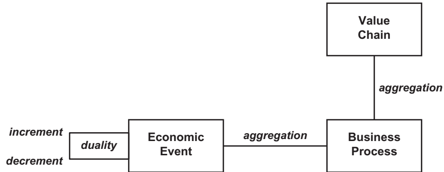
FIGURE 4-9(a) Class Diagram of REA Granularity Levels 2-3
