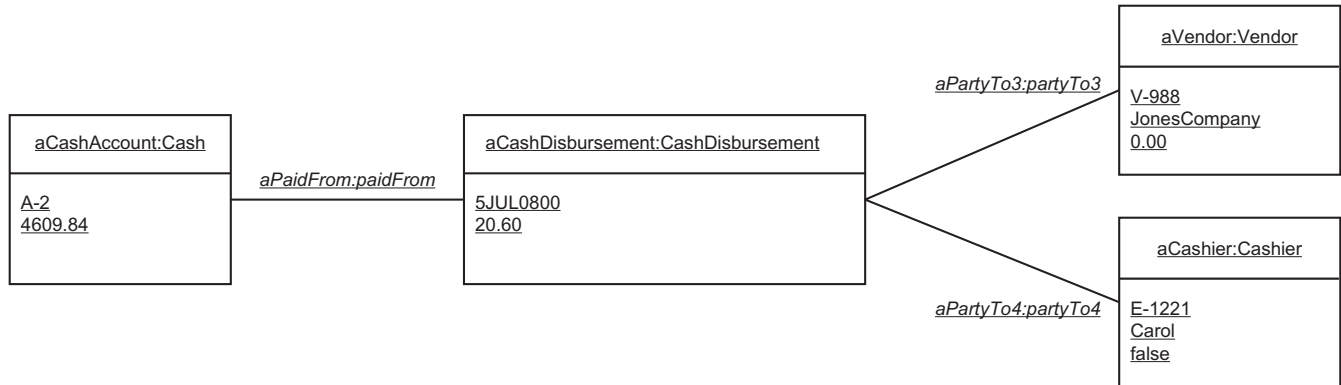
(c) – REA Pattern at Level-M0 – An REA Instantiation
