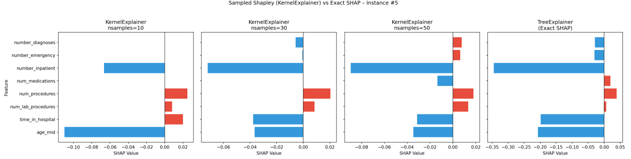
Figure 5. Sampled Shapley (KernelExplainer) vs. Exact SHAP (TreeExplainer) Across Path Counts. The three left panels show KernelExplainer attributions at n_{\text{samples}} = 10, 30 , and 50 for a single test instance. The rightmost panel shows the exact TreeExplainer values as the reference standard. Attribution direction is consistent across all configurations; magnitude converges toward the exact values as n_{\text{samples}} increases.
