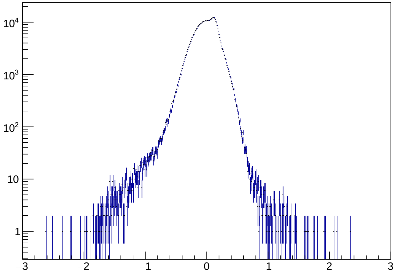
Photon Seed Time Calibrated [ns]
