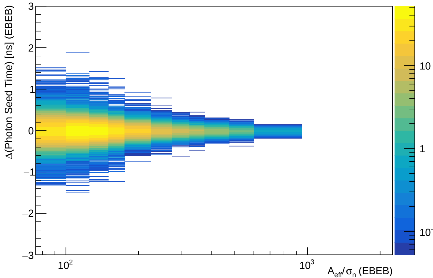
\Delta(\text{Photon Seed Time}) [\text{ns}] vs. A_{\text{eff}}/\sigma_n (EBEB)
