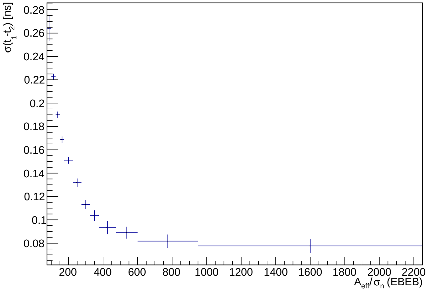
\Delta(\text{Photon Seed Time}) [ns] vs. A_{\text{eff}}/\sigma_n (EBEB) \sigma(t_1-t_2) [ns]
