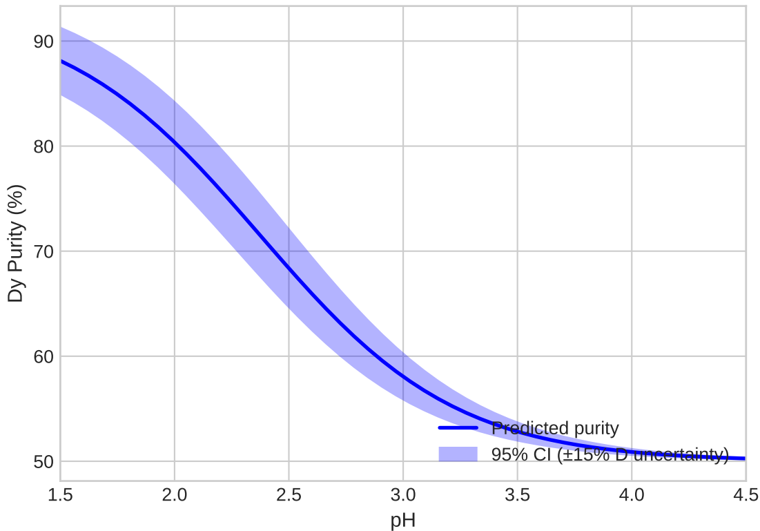
Purity Prediction with D Coefficient Uncertainty
