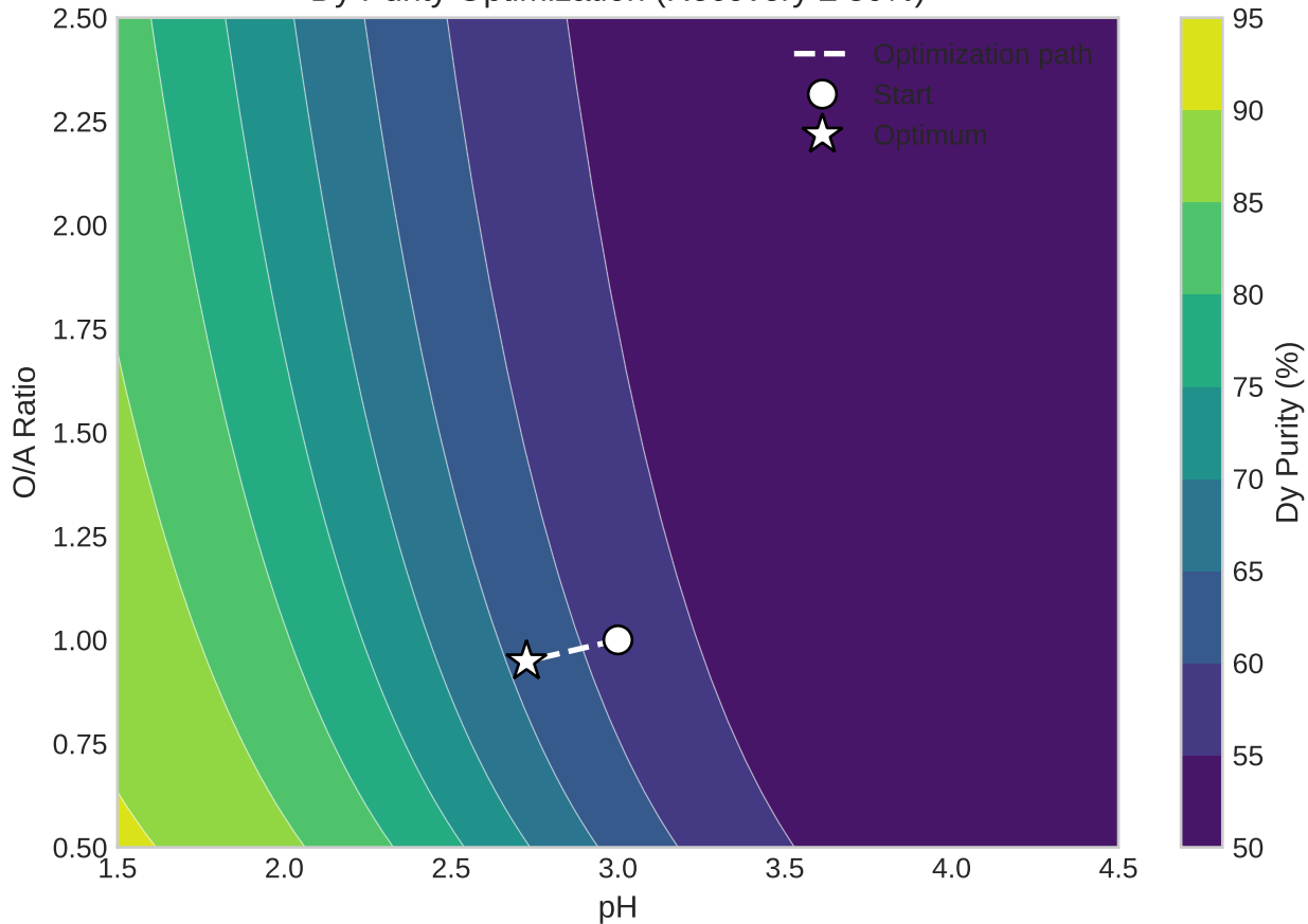
Dy Purity Optimization (Recovery \geq 80\% )
