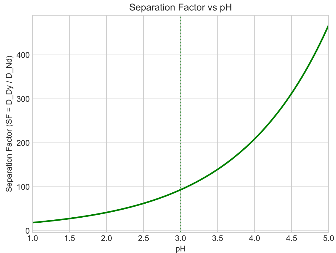
Figure 2: D2EHPA Extraction (0.5 M, 25°C)
