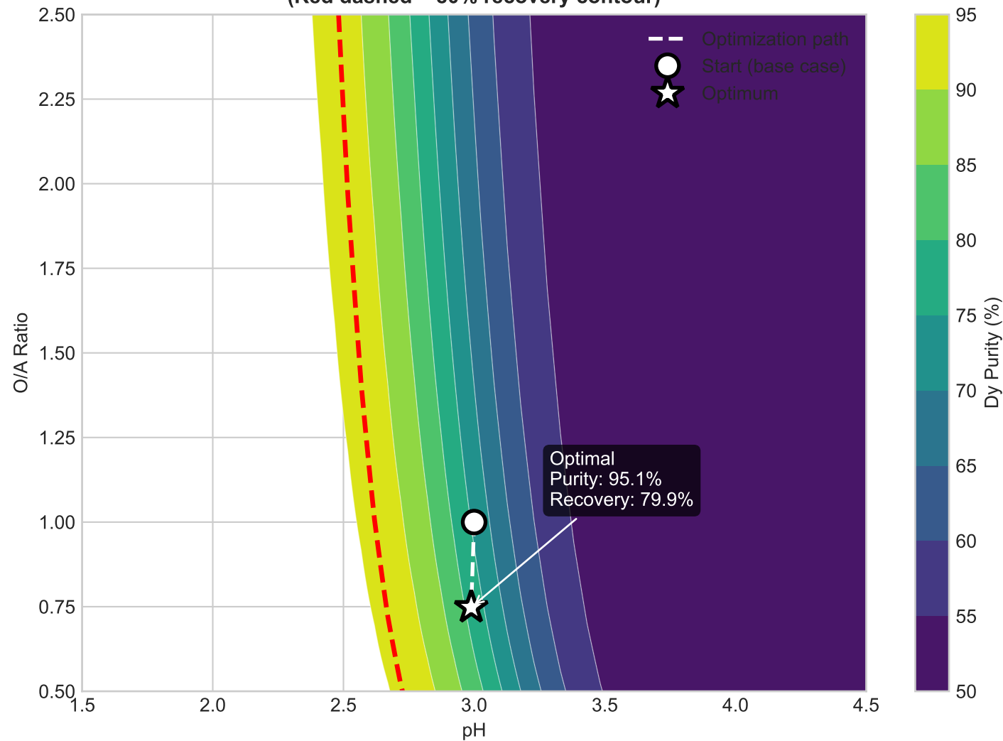
Figure 3: Purity Optimization with Recovery \geq 80\% Constraint (Red dashed = 80% recovery contour)
